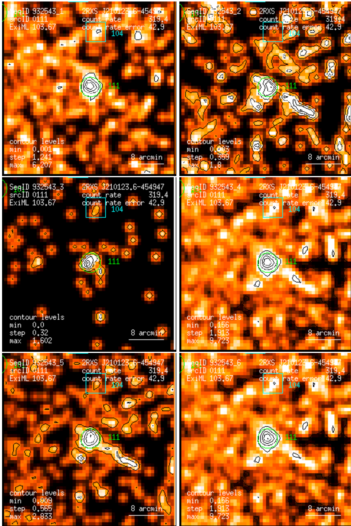
Figure 111: RASS 932543: detection 0111: band rate images, Gaussian filter: (1) PSPC channels 11 – 41, (2) 52 – 90, (3) 91 – 201, (4) 11 – 235, (5) 52 – 201, (6) 11 – 201. Broad band rates in counts/ks. Band rate contour levels in counts/ks/arcmin 2 .
