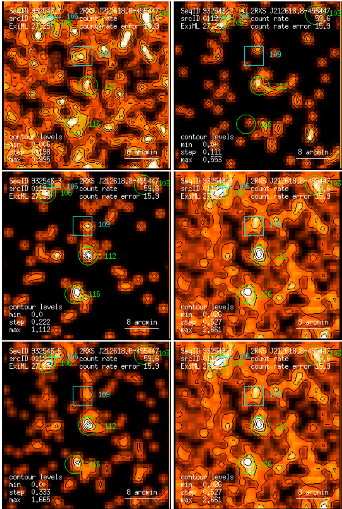
Figure 112: RASS 932543: detection 0112: band rate images, Gaussian filter: (1) PSPC channels 11 – 41, (2) 52 – 90, (3) 91 – 201, (4) 11 – 235, (5) 52 – 201, (6) 11 – 201. Broad band rates in counts/ks. Band rate contour levels in counts/ks/arcmin 2 .
