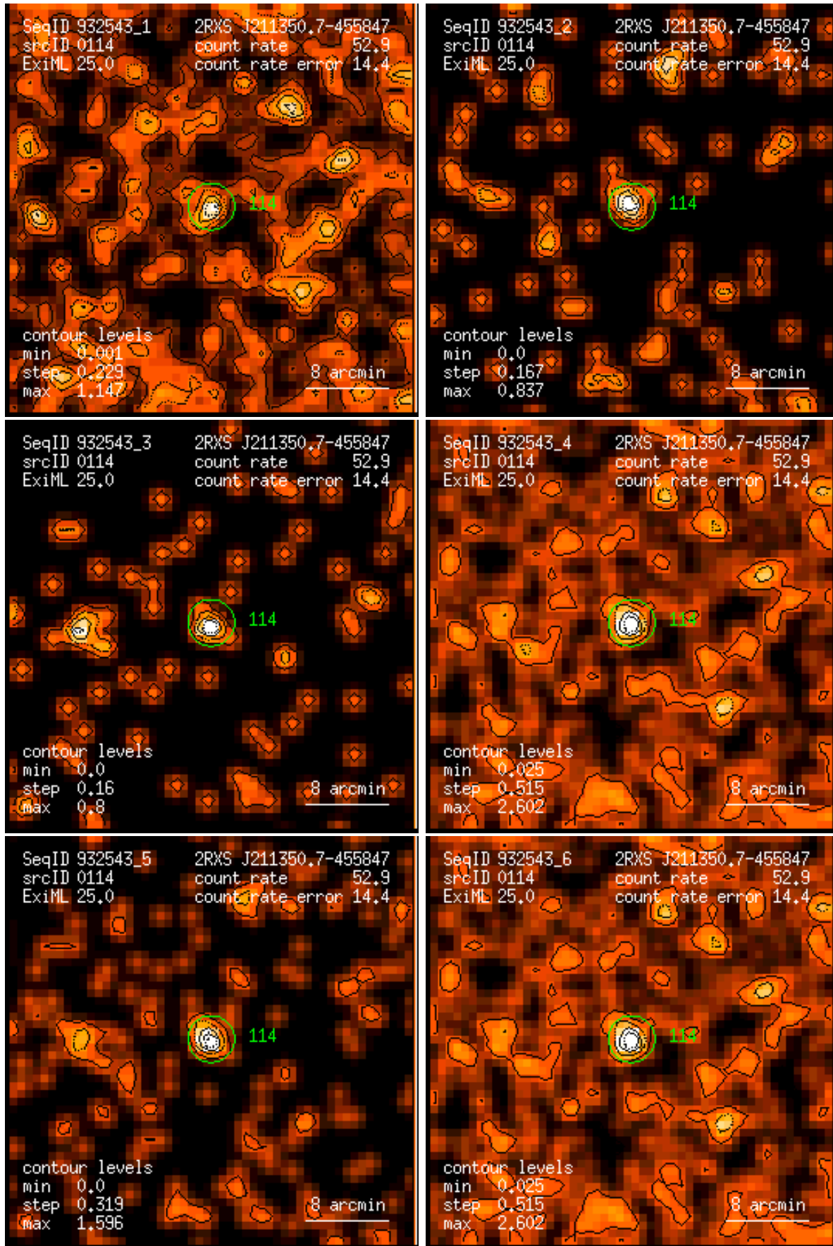
Figure 114: RASS 932543: detection 0114: band rate images, Gaussian filter: (1) PSPC channels 11 – 41, (2) 52 – 90, (3) 91 – 201, (4) 11 – 235, (5) 52 – 201, (6) 11 – 201. Broad band rates in counts/ks. Band rate contour levels in counts/ks/arcmin 2 .
