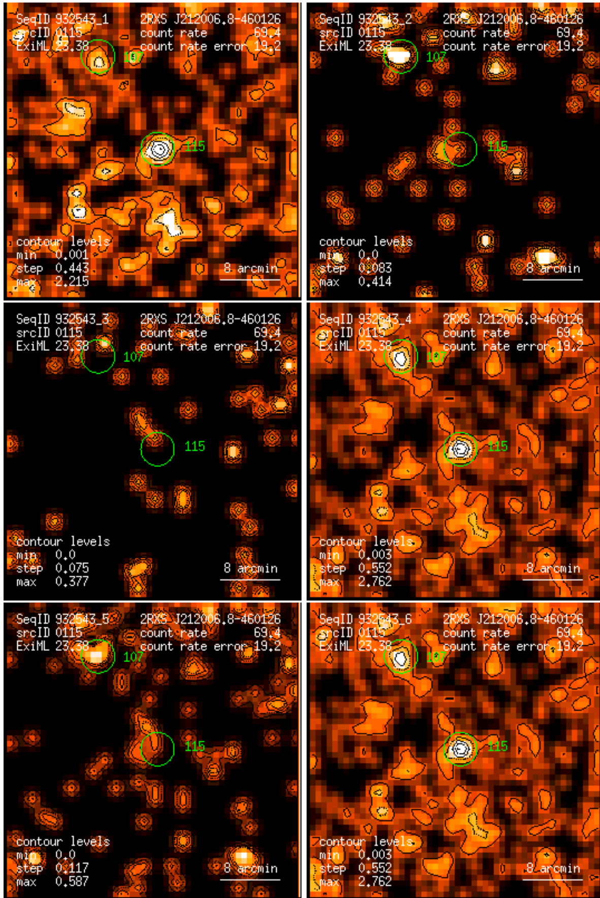
Figure 115: RASS 932543: detection 0115: band rate images, Gaussian filter: (1) PSPC channels 11 – 41, (2) 52 – 90, (3) 91 – 201, (4) 11 – 235, (5) 52 – 201, (6) 11 – 201. Broad band rates in counts/ks. Band rate contour levels in counts/ks/arcmin 2 .
