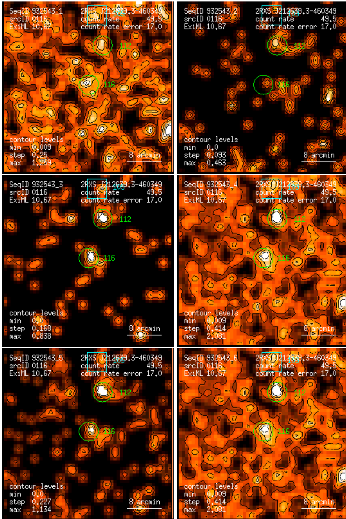
Figure 116: RASS 932543: detection 0116: band rate images, Gaussian filter: (1) PSPC channels 11 – 41, (2) 52 – 90, (3) 91 – 201, (4) 11 – 235, (5) 52 – 201, (6) 11 – 201. Broad band rates in counts/ks. Band rate contour levels in counts/ks/arcmin 2 .
