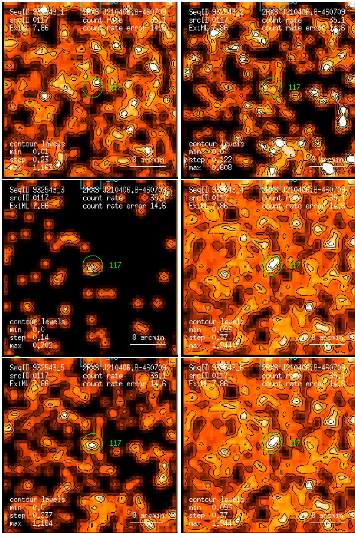
Figure 117: RASS 932543: detection 0117: band rate images, Gaussian filter: (1) PSPC channels 11 – 41, (2) 52 – 90, (3) 91 – 201, (4) 11 – 235, (5) 52 – 201, (6) 11 – 201. Broad band rates in counts/ks. Band rate contour levels in counts/ks/arcmin 2 .
