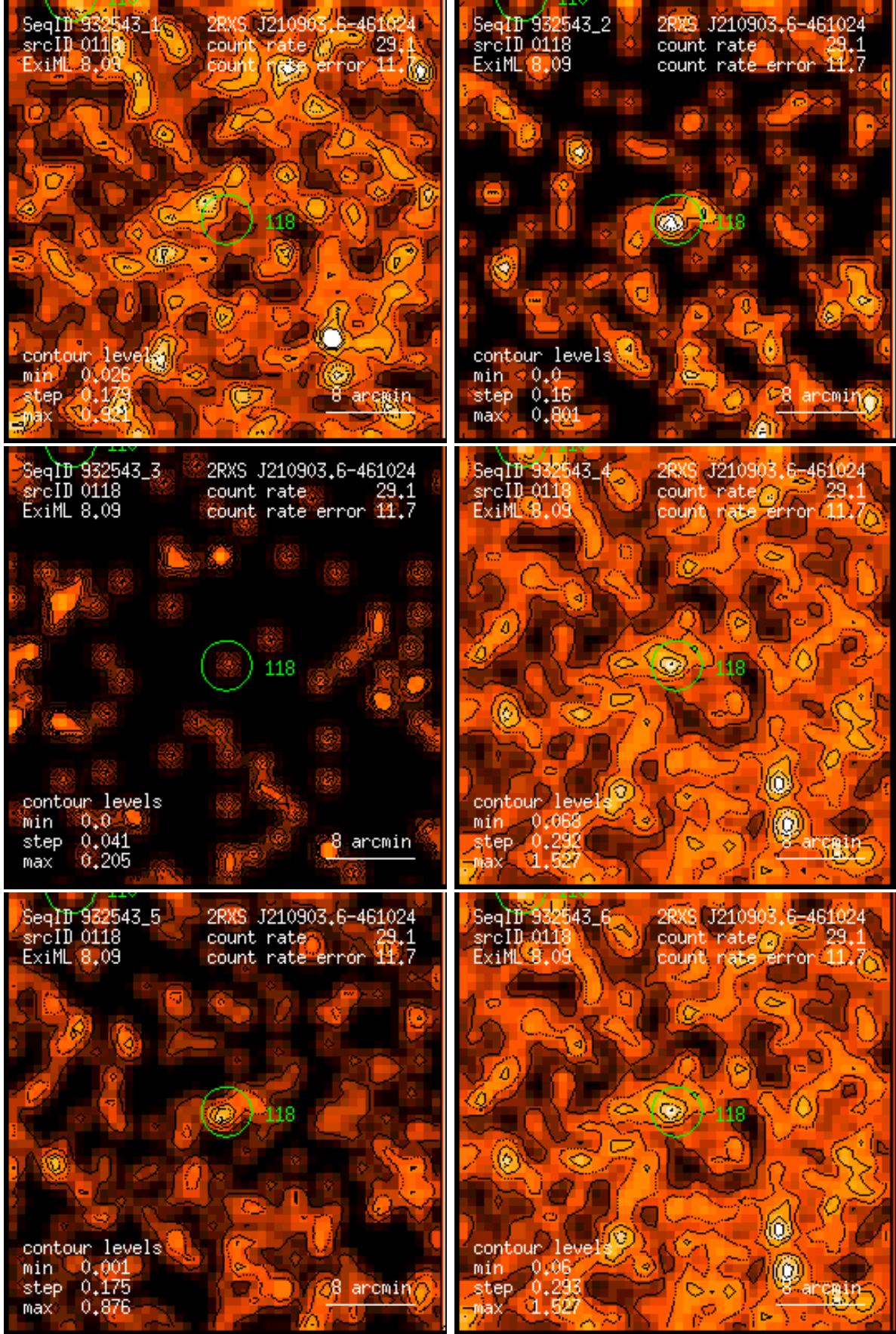
Figure 118: RASS 932543: detection 0118: band rate images, Gaussian filter: (1) PSPC channels 11 – 41, (2) 52 – 90, (3) 91 – 201, (4) 11 – 235, (5) 52 – 201, (6) 11 – 201. Broad band rates in counts/ks. Band rate contour levels in counts/ks/arcmin 2 .
