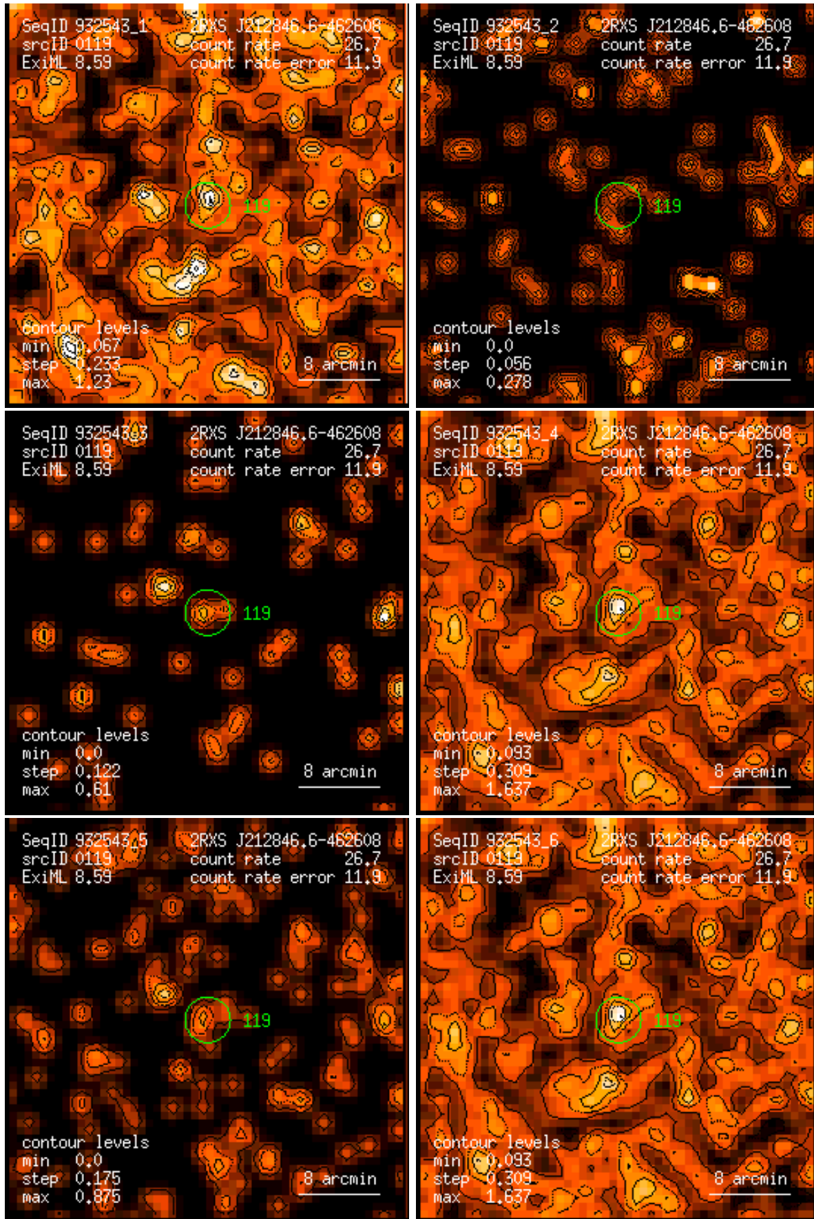
Figure 119: RASS 932543: detection 0119: band rate images, Gaussian filter: (1) PSPC channels 11 – 41, (2) 52 – 90, (3) 91 – 201, (4) 11 – 235, (5) 52 – 201, (6) 11 – 201. Broad band rates in counts/ks. Band rate contour levels in counts/ks/arcmin 2 .
