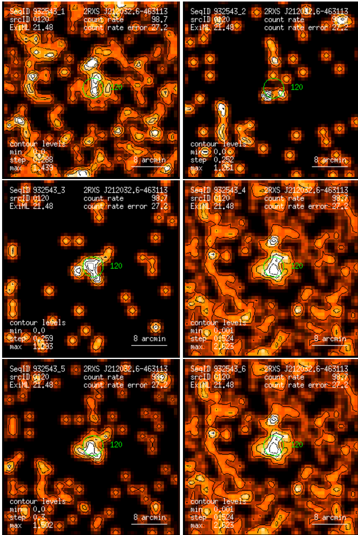
Figure 120: RASS 932543: detection 0120: band rate images, Gaussian filter: (1) PSPC channels 11 – 41, (2) 52 – 90, (3) 91 – 201, (4) 11 – 235, (5) 52 – 201, (6) 11 – 201. Broad band rates in counts/ks. Band rate contour levels in counts/ks/arcmin 2 .
