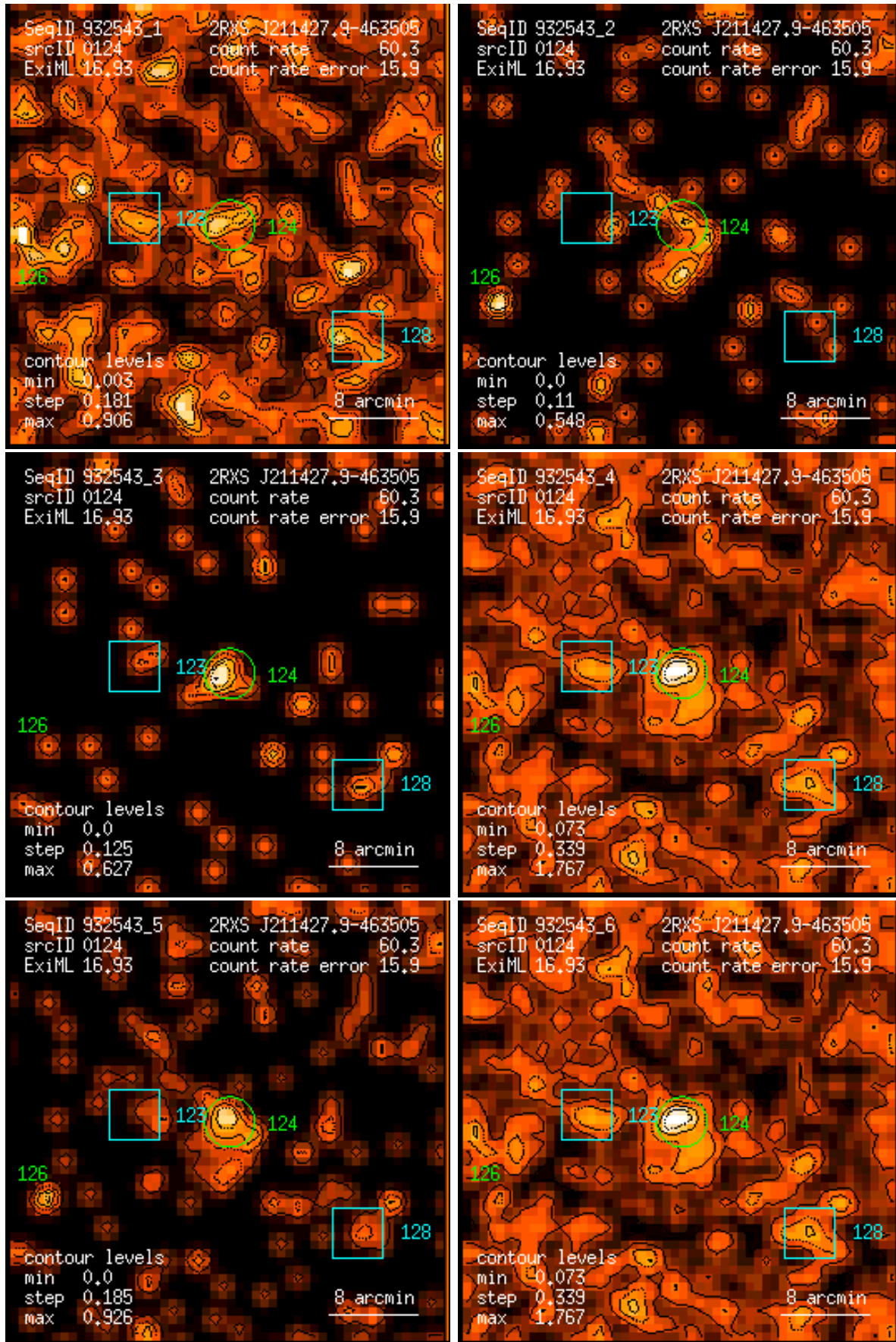
Figure 124: RASS 932543: detection 0124: band rate images, Gaussian filter: (1) PSPC channels 11 – 41, (2) 52 – 90, (3) 91 – 201, (4) 11 – 235, (5) 52 – 201, (6) 11 – 201. Broad band rates in counts/ks. Band rate contour levels in counts/ks/arcmin 2 .
