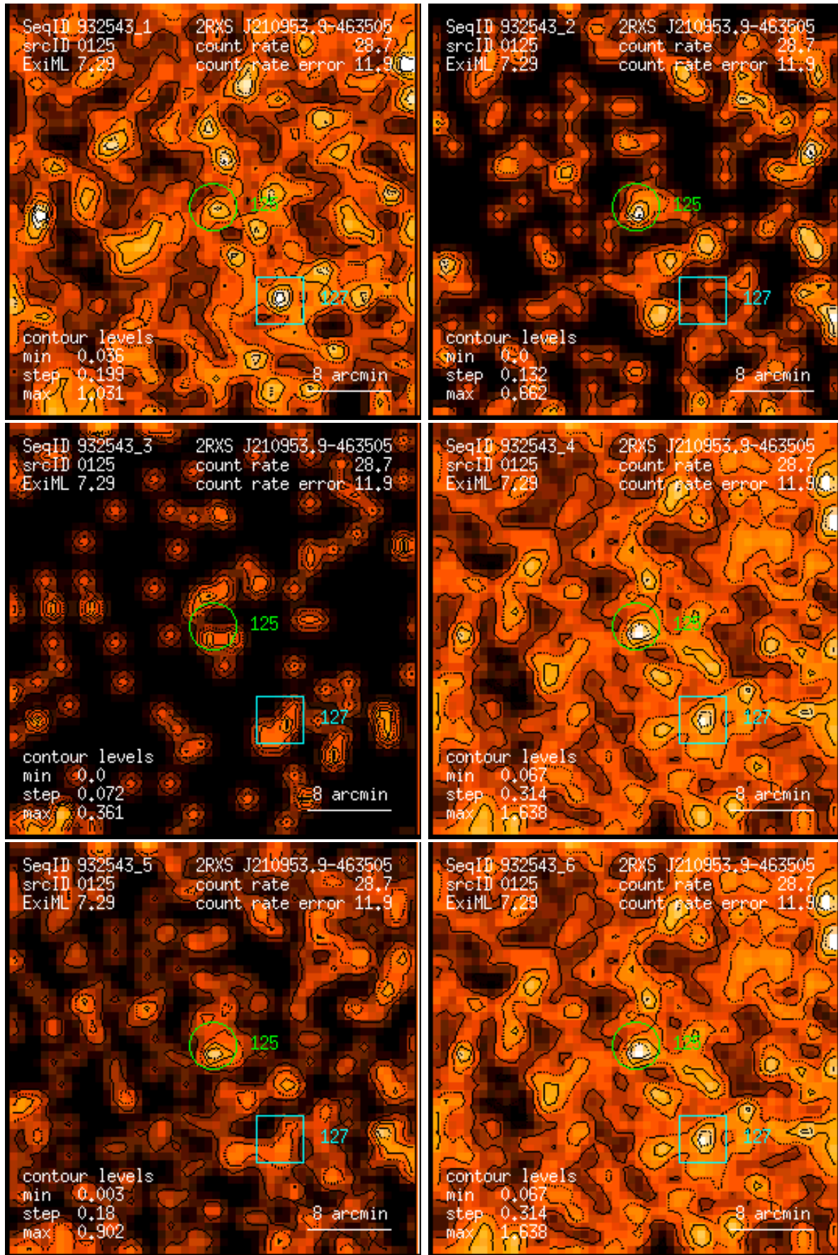
Figure 125: RASS 932543: detection 0125: band rate images, Gaussian filter: (1) PSPC channels 11 – 41, (2) 52 – 90, (3) 91 – 201, (4) 11 – 235, (5) 52 – 201, (6) 11 – 201. Broad band rates in counts/ks. Band rate contour levels in counts/ks/arcmin 2 .
