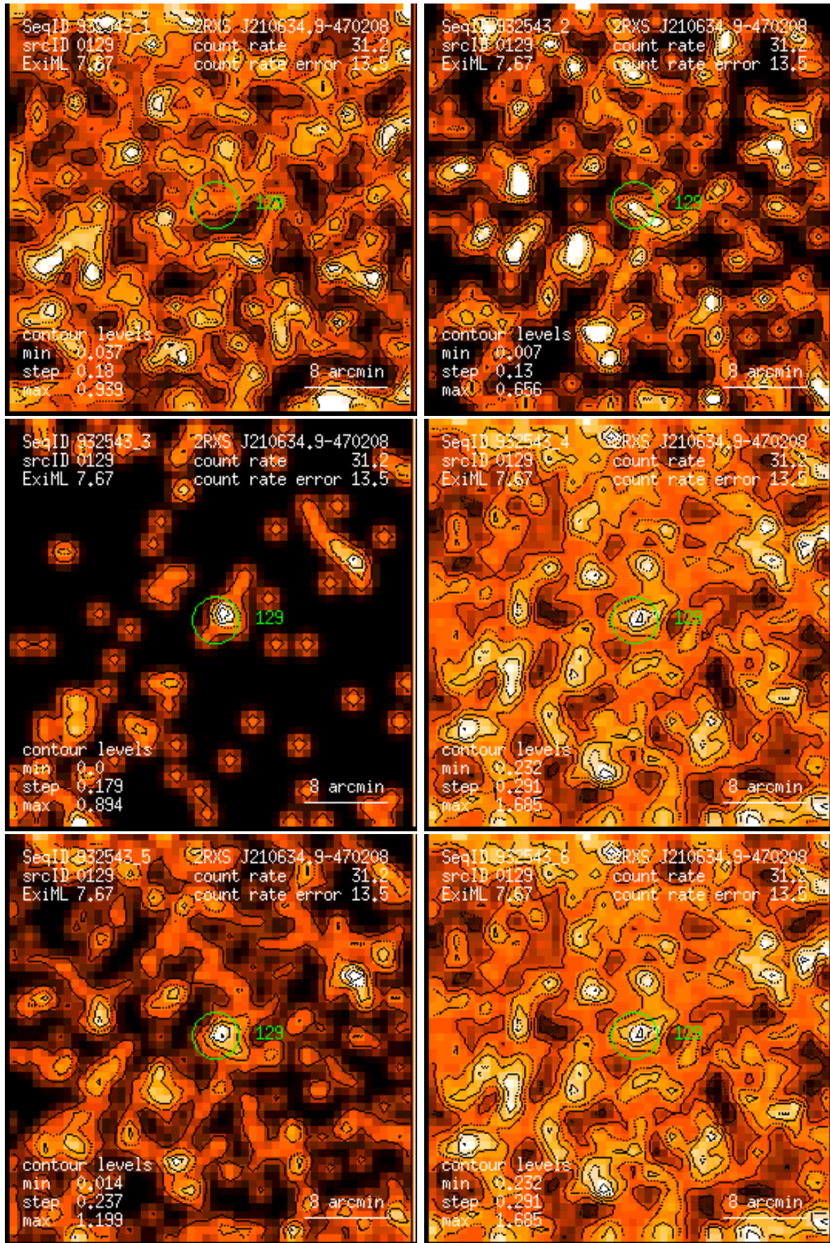
Figure 129: RASS 932543: detection 0129: band rate images, Gaussian filter: (1) PSPC channels 11 – 41, (2) 52 – 90, (3) 91 – 201, (4) 11 – 235, (5) 52 – 201, (6) 11 – 201. Broad band rates in counts/ks. Band rate contour levels in counts/ks/arcmin 2 .
