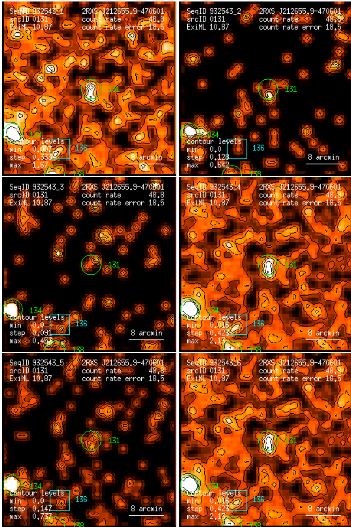
Figure 131: RASS 932543: detection 0131: band rate images, Gaussian filter: (1) PSPC channels 11 – 41, (2) 52 – 90, (3) 91 – 201, (4) 11 – 235, (5) 52 – 201, (6) 11 – 201. Broad band rates in counts/ks. Band rate contour levels in counts/ks/arcmin 2 .
