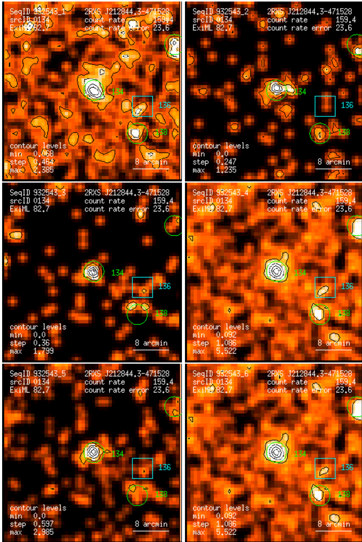
Figure 134: RASS 932543: detection 0134: band rate images, Gaussian filter: (1) PSPC channels 11 – 41, (2) 52 – 90, (3) 91 – 201, (4) 11 – 235, (5) 52 – 201, (6) 11 – 201. Broad band rates in counts/ks. Band rate contour levels in counts/ks/arcmin 2 .
