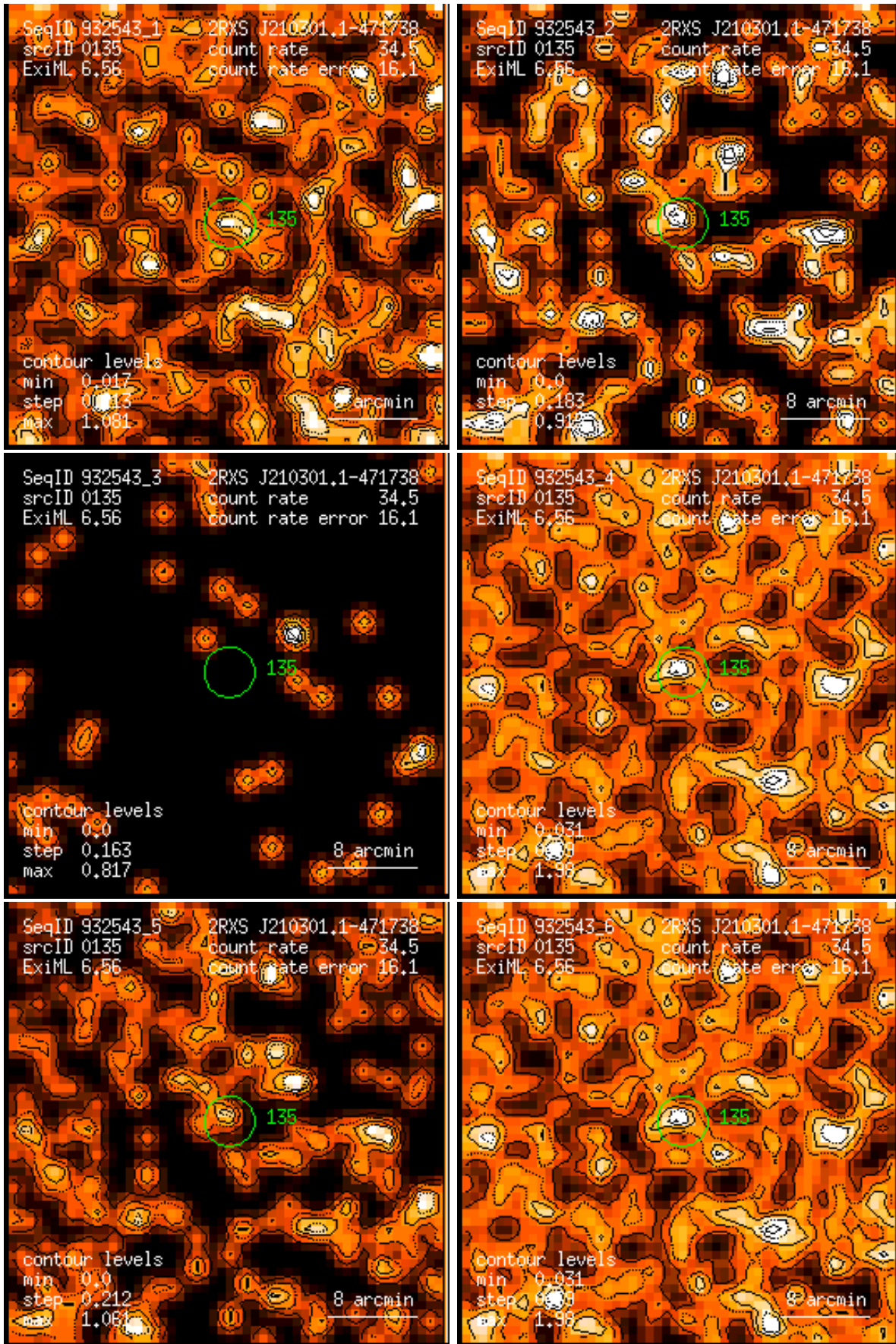
Figure 135: RASS 932543: detection 0135: band rate images, Gaussian filter: (1) PSPC channels 11 – 41, (2) 52 – 90, (3) 91 – 201, (4) 11 – 235, (5) 52 – 201, (6) 11 – 201. Broad band rates in counts/ks. Band rate contour levels in counts/ks/arcmin 2 .
