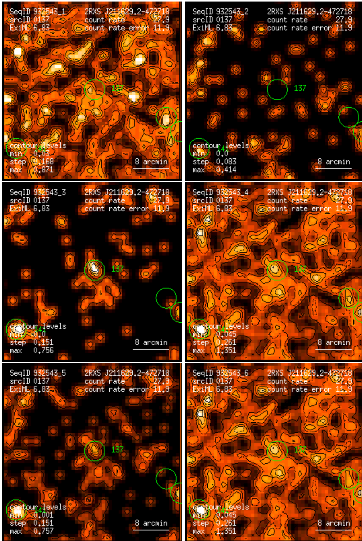
Figure 137: RASS 932543: detection 0137: band rate images, Gaussian filter: (1) PSPC channels 11 – 41, (2) 52 – 90, (3) 91 – 201, (4) 11 – 235, (5) 52 – 201, (6) 11 – 201. Broad band rates in counts/ks. Band rate contour levels in counts/ks/arcmin 2 .
