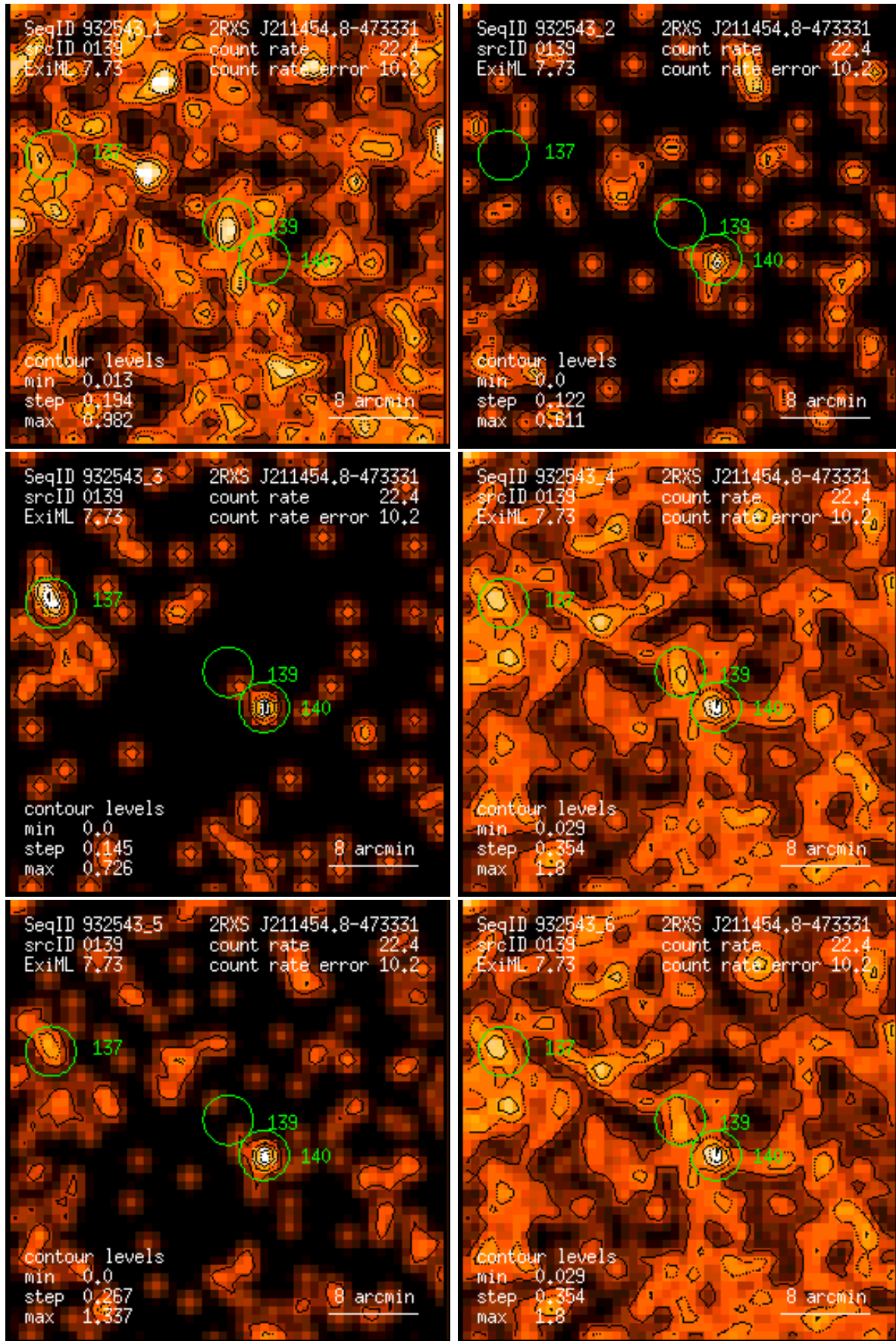
Figure 139: RASS 932543: detection 0139: band rate images, Gaussian filter: (1) PSPC channels 11 – 41, (2) 52 – 90, (3) 91 – 201, (4) 11 – 235, (5) 52 – 201, (6) 11 – 201. Broad band rates in counts/ks. Band rate contour levels in counts/ks/arcmin 2 .
