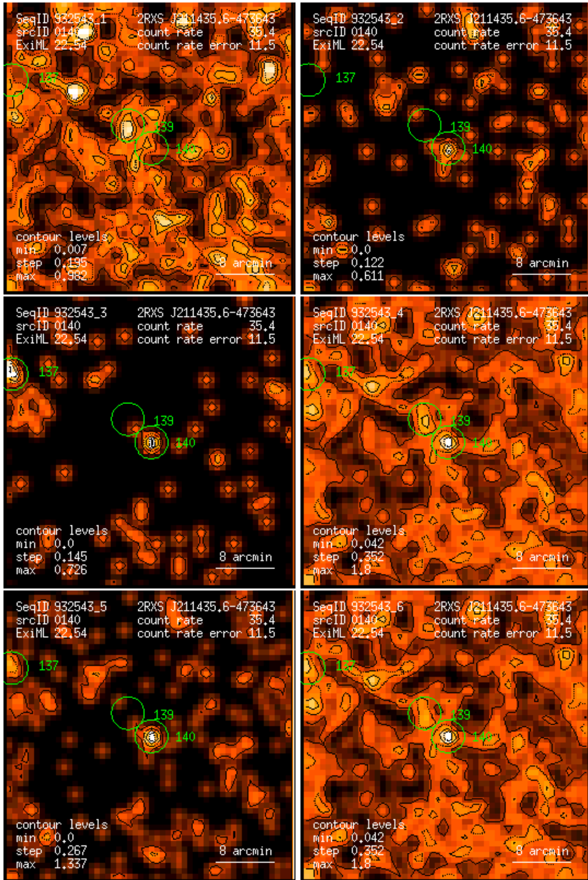
Figure 140: RASS 932543: detection 0140: band rate images, Gaussian filter: (1) PSPC channels 11 – 41, (2) 52 – 90, (3) 91 – 201, (4) 11 – 235, (5) 52 – 201, (6) 11 – 201. Broad band rates in counts/ks. Band rate contour levels in counts/ks/arcmin 2 .
