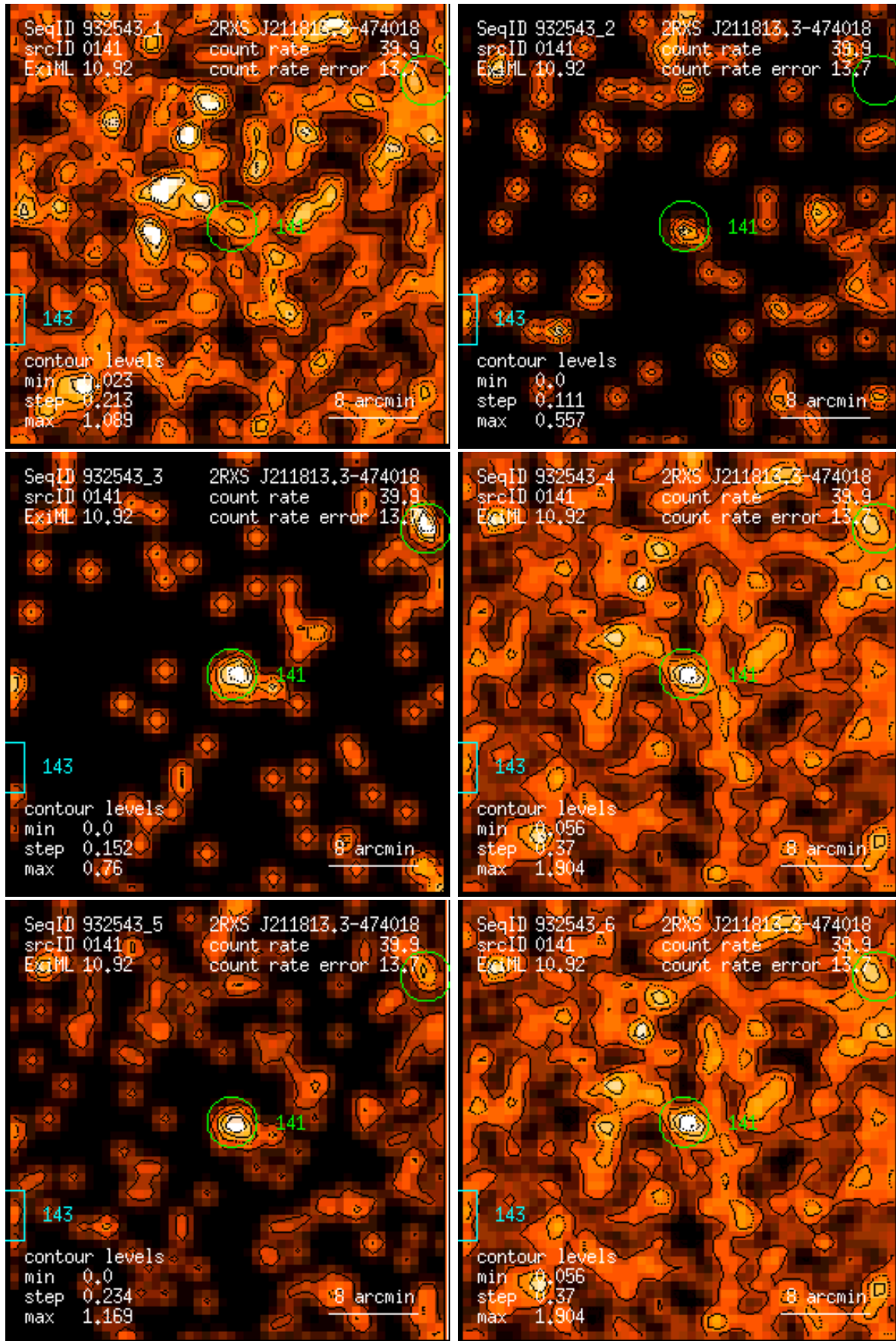
Figure 141: RASS 932543: detection 0141: band rate images, Gaussian filter: (1) PSPC channels 11 – 41, (2) 52 – 90, (3) 91 – 201, (4) 11 – 235, (5) 52 – 201, (6) 11 – 201. Broad band rates in counts/ks. Band rate contour levels in counts/ks/arcmin 2 .
