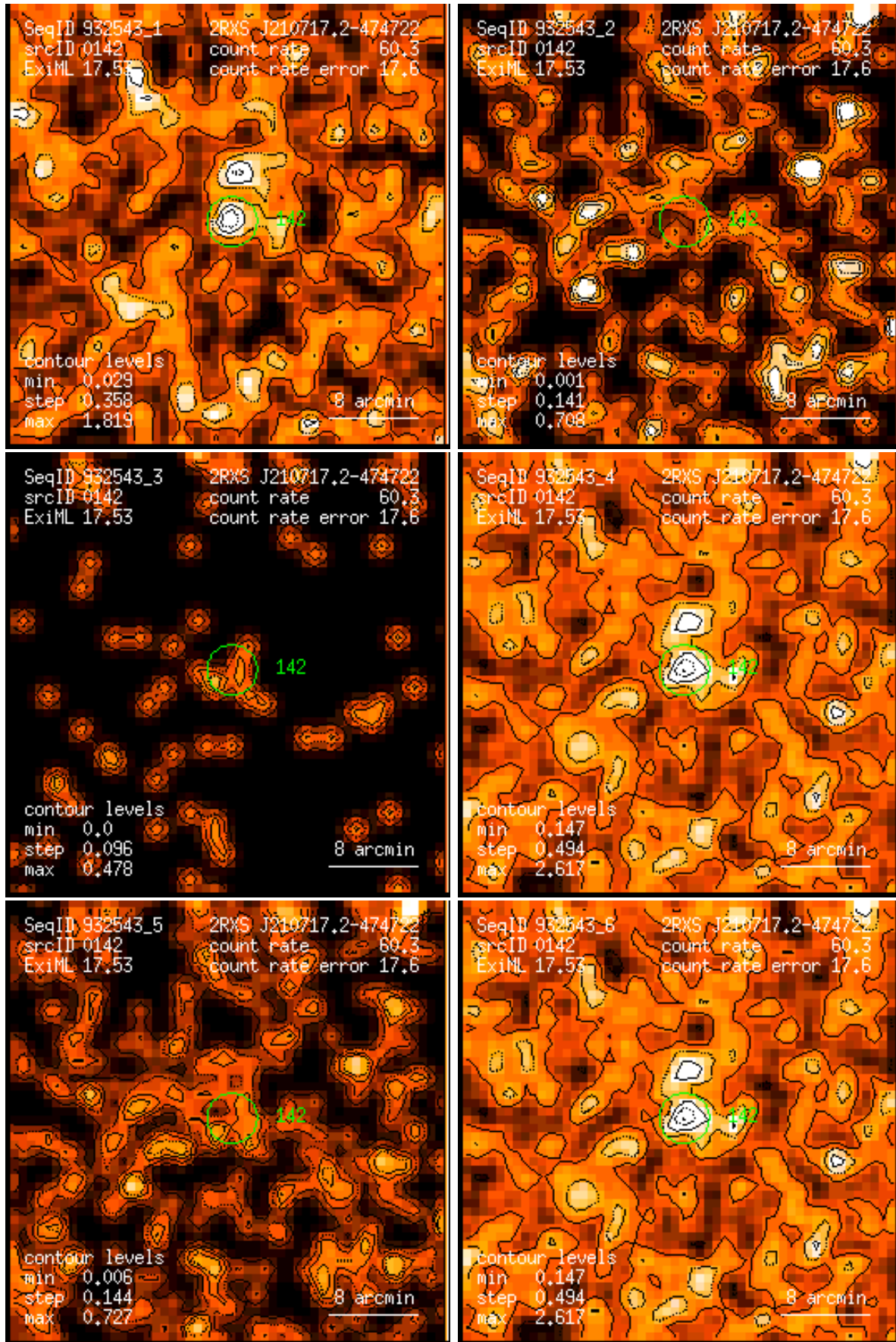
Figure 142: RASS 932543: detection 0142: band rate images, Gaussian filter: (1) PSPC channels 11 – 41, (2) 52 – 90, (3) 91 – 201, (4) 11 – 235, (5) 52 – 201, (6) 11 – 201. Broad band rates in counts/ks. Band rate contour levels in counts/ks/arcmin 2 .
