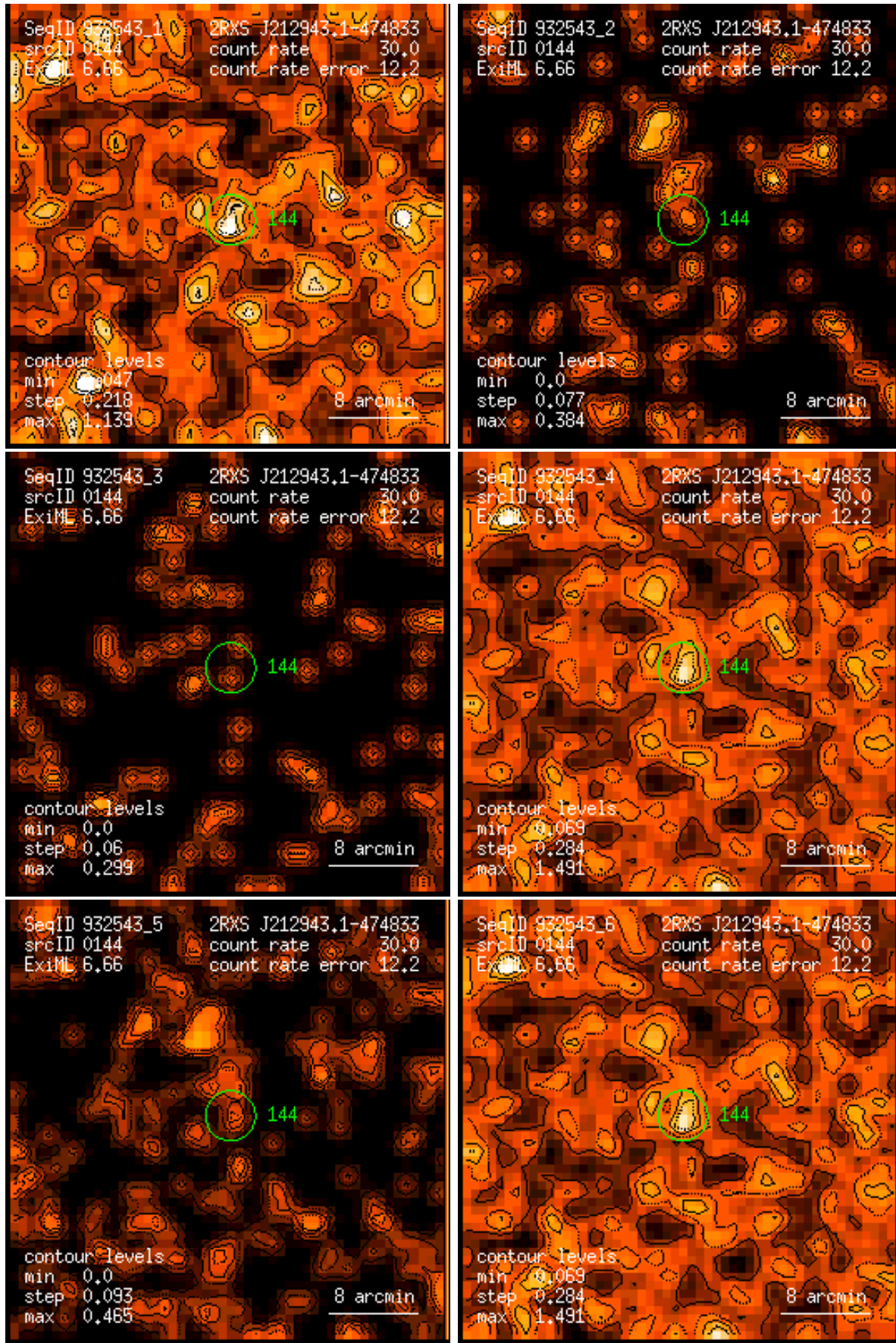
Figure 144: RASS 932543: detection 0144: band rate images, Gaussian filter: (1) PSPC channels 11 – 41, (2) 52 – 90, (3) 91 – 201, (4) 11 – 235, (5) 52 – 201, (6) 11 – 201. Broad band rates in counts/ks. Band rate contour levels in counts/ks/arcmin 2 .
