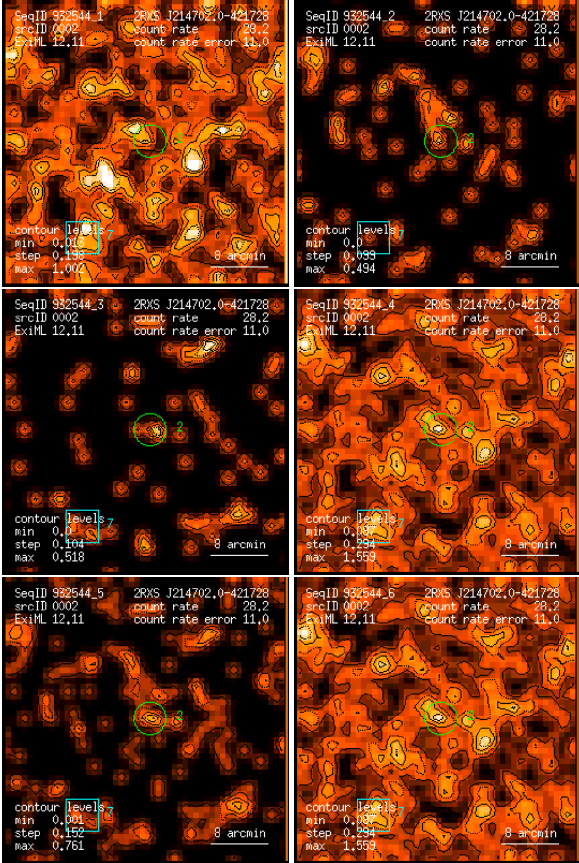
Figure 2: RASS 932544: detection 0002: band rate images, Gaussian filter: (1) PSPC channels 11 – 41, (2) 52 – 90, (3) 91 – 201, (4) 11 – 235, (5) 52 – 201, (6) 11 – 201. Broad band rates in counts/ks. Band rate contour levels in counts/ks/arcmin 2 .
