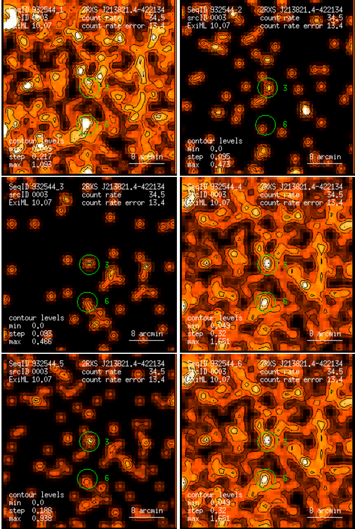
Figure 3: RASS 932544: detection 0003: band rate images, Gaussian filter: (1) PSPC channels 11 – 41, (2) 52 – 90, (3) 91 – 201, (4) 11 – 235, (5) 52 – 201, (6) 11 – 201. Broad band rates in counts/ks. Band rate contour levels in counts/ks/arcmin 2 .
