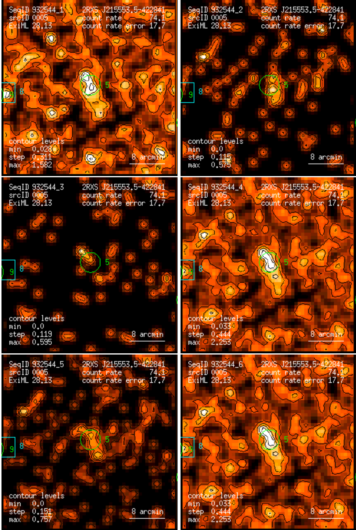
Figure 5: RASS 932544: detection 0005: band rate images, Gaussian filter: (1) PSPC channels 11 – 41, (2) 52 – 90, (3) 91 – 201, (4) 11 – 235, (5) 52 – 201, (6) 11 – 201. Broad band rates in counts/ks. Band rate contour levels in counts/ks/arcmin 2 .
