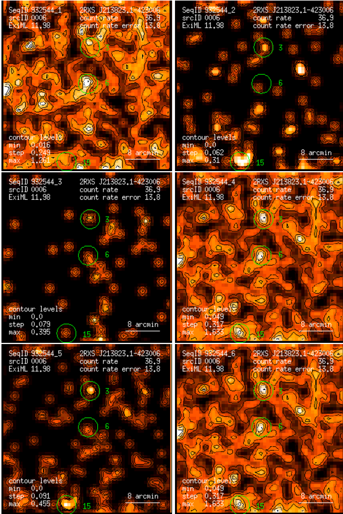
Figure 6: RASS 932544: detection 0006: band rate images, Gaussian filter: (1) PSPC channels 11 – 41, (2) 52 – 90, (3) 91 – 201, (4) 11 – 235, (5) 52 – 201, (6) 11 – 201. Broad band rates in counts/ks. Band rate contour levels in counts/ks/arcmin 2 .
