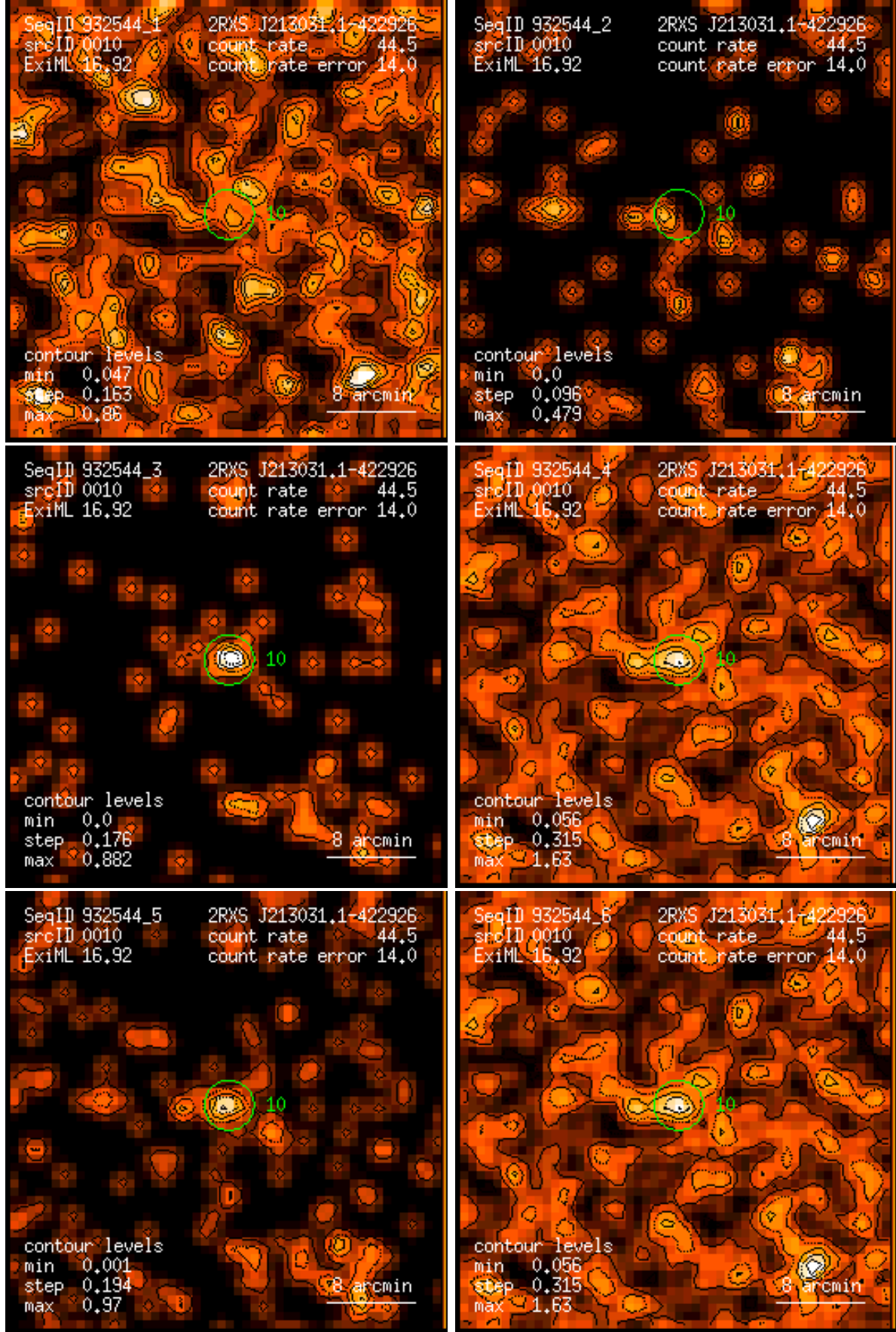
Figure 10: RASS 932544: detection 0010: band rate images, Gaussian filter: (1) PSPC channels 11 – 41, (2) 52 – 90, (3) 91 – 201, (4) 11 – 235, (5) 52 – 201, (6) 11 – 201. Broad band rates in counts/ks. Band rate contour levels in counts/ks/arcmin 2 .
