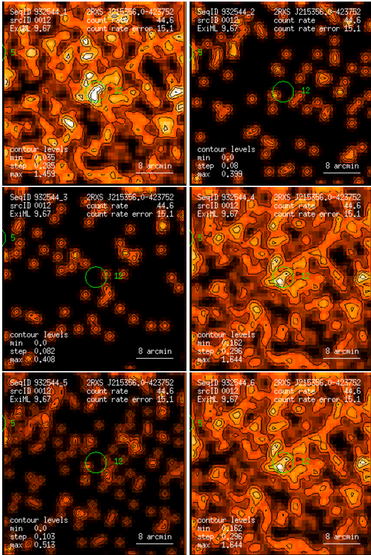
Figure 12: RASS 932544: detection 0012: band rate images, Gaussian filter: (1) PSPC channels 11 – 41, (2) 52 – 90, (3) 91 – 201, (4) 11 – 235, (5) 52 – 201, (6) 11 – 201. Broad band rates in counts/ks. Band rate contour levels in counts/ks/arcmin 2 .
