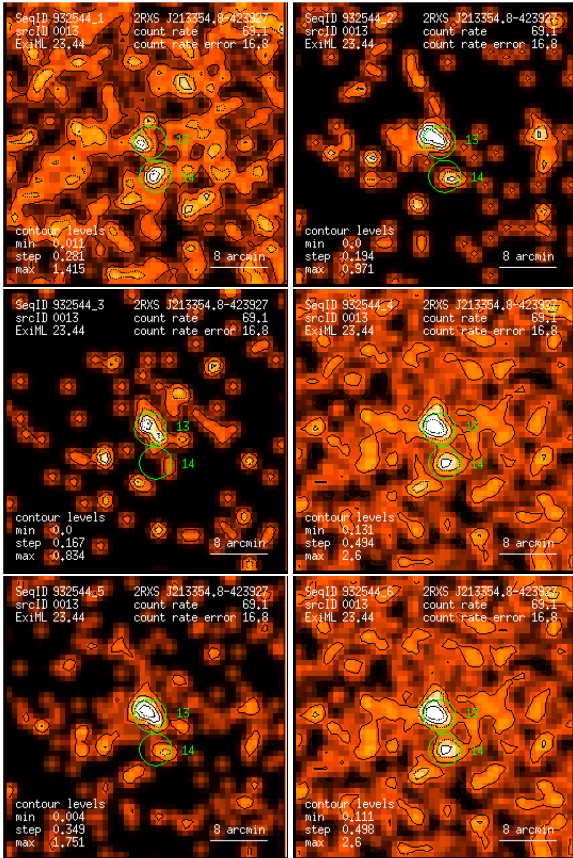
Figure 13: RASS 932544: detection 0013: band rate images, Gaussian filter: (1) PSPC channels 11 – 41, (2) 52 – 90, (3) 91 – 201, (4) 11 – 235, (5) 52 – 201, (6) 11 – 201. Broad band rates in counts/ks. Band rate contour levels in counts/ks/arcmin 2 .
