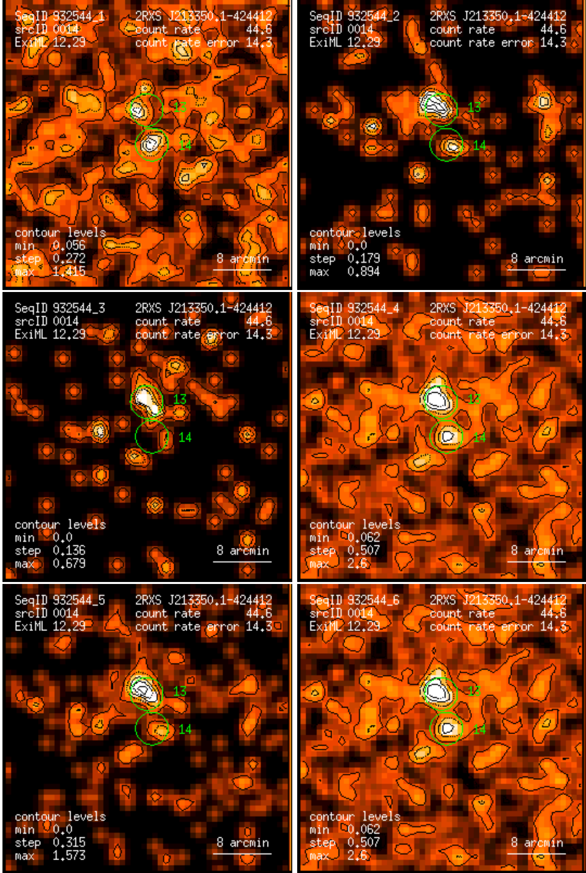
Figure 14: RASS 932544: detection 0014: band rate images, Gaussian filter: (1) PSPC channels 11 – 41, (2) 52 – 90, (3) 91 – 201, (4) 11 – 235, (5) 52 – 201, (6) 11 – 201. Broad band rates in counts/ks. Band rate contour levels in counts/ks/arcmin 2 .
