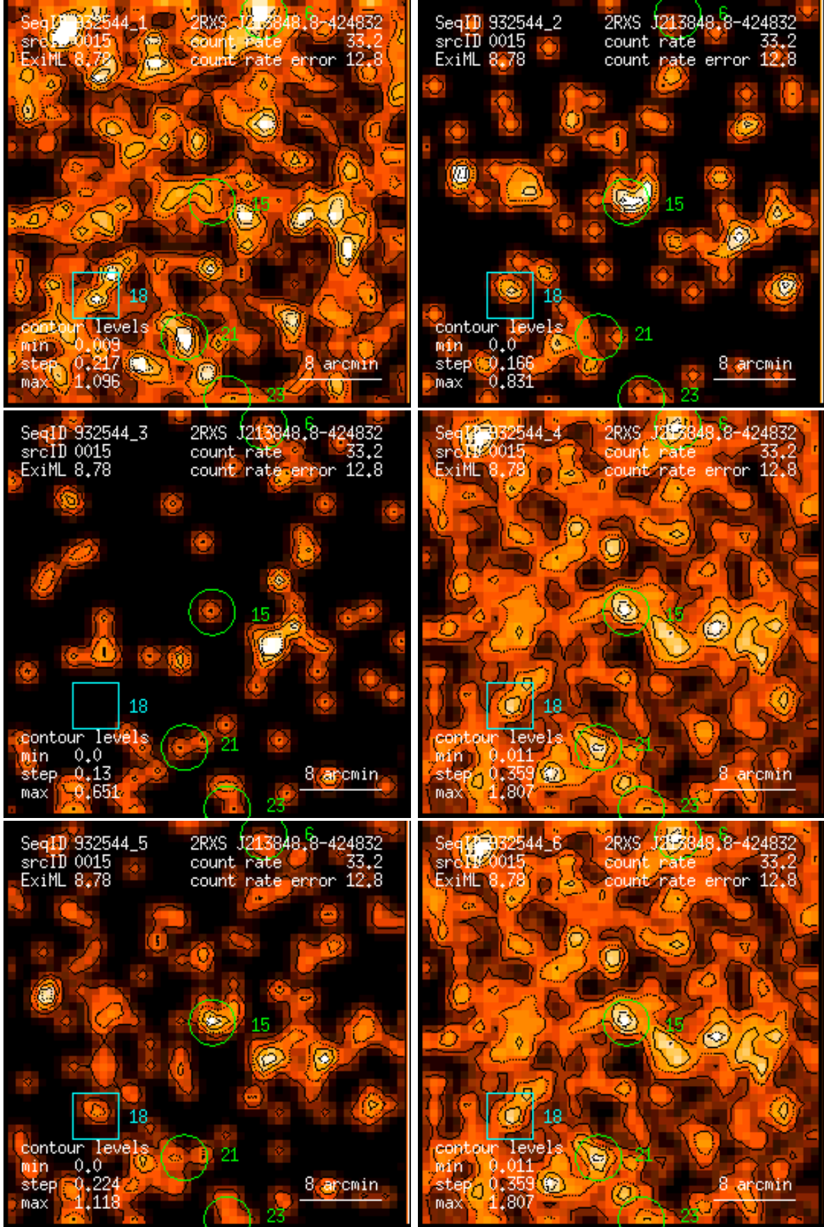
Figure 15: RASS 932544: detection 0015: band rate images, Gaussian filter: (1) PSPC channels 11 – 41, (2) 52 – 90, (3) 91 – 201, (4) 11 – 235, (5) 52 – 201, (6) 11 – 201. Broad band rates in counts/ks. Band rate contour levels in counts/ks/arcmin 2 .
