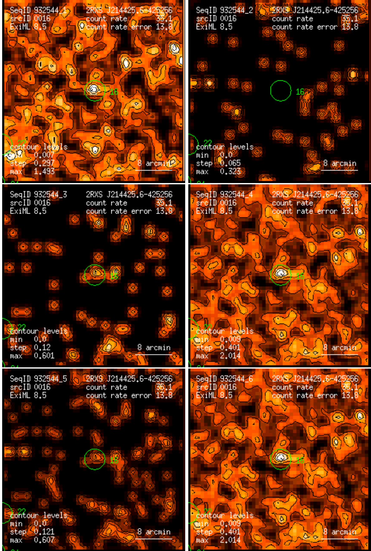
Figure 16: RASS 932544: detection 0016: band rate images, Gaussian filter: (1) PSPC channels 11 – 41, (2) 52 – 90, (3) 91 – 201, (4) 11 – 235, (5) 52 – 201, (6) 11 – 201. Broad band rates in counts/ks. Band rate contour levels in counts/ks/arcmin 2 .
