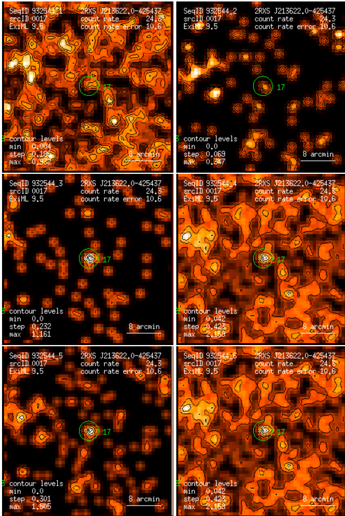
Figure 17: RASS 932544: detection 0017: band rate images, Gaussian filter: (1) PSPC channels 11 – 41, (2) 52 – 90, (3) 91 – 201, (4) 11 – 235, (5) 52 – 201, (6) 11 – 201. Broad band rates in counts/ks. Band rate contour levels in counts/ks/arcmin 2 .
