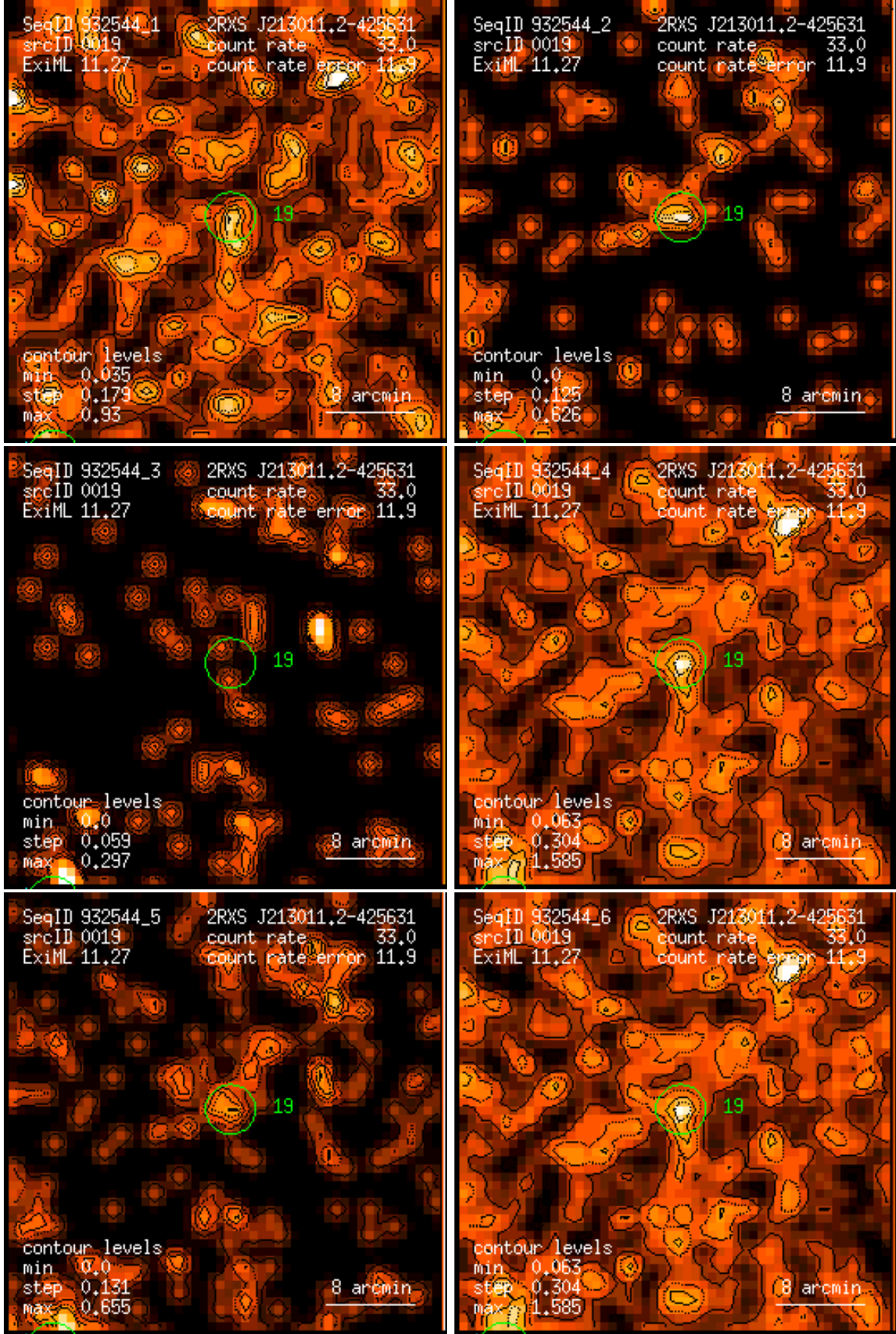
Figure 19: RASS 932544: detection 0019: band rate images, Gaussian filter: (1) PSPC channels 11 – 41, (2) 52 – 90, (3) 91 – 201, (4) 11 – 235, (5) 52 – 201, (6) 11 – 201. Broad band rates in counts/ks. Band rate contour levels in counts/ks/arcmin 2 .
