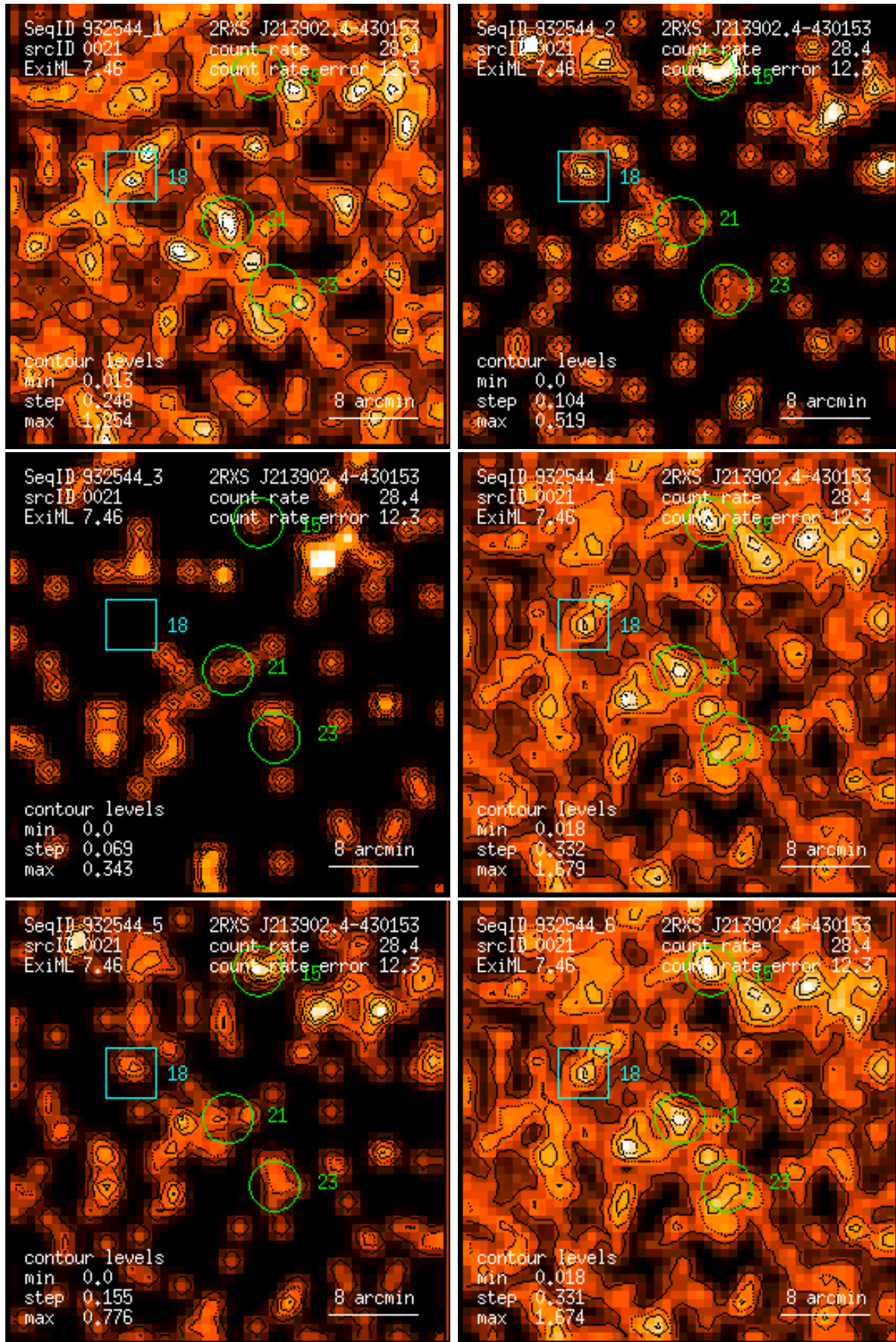
Figure 21: RASS 932544: detection 0021: band rate images, Gaussian filter: (1) PSPC channels 11 – 41, (2) 52 – 90, (3) 91 – 201, (4) 11 – 235, (5) 52 – 201, (6) 11 – 201. Broad band rates in counts/ks. Band rate contour levels in counts/ks/arcmin 2 .
