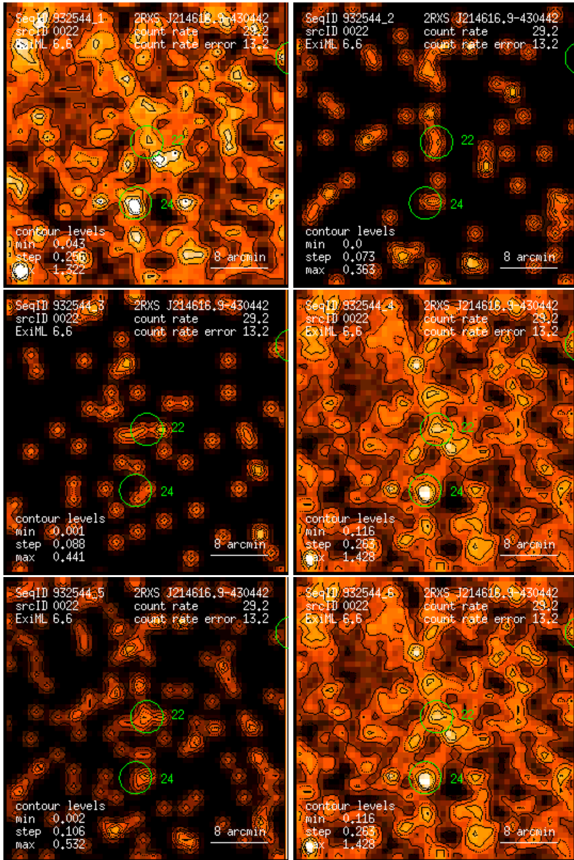
Figure 22: RASS 932544: detection 0022: band rate images, Gaussian filter: (1) PSPC channels 11 – 41, (2) 52 – 90, (3) 91 – 201, (4) 11 – 235, (5) 52 – 201, (6) 11 – 201. Broad band rates in counts/ks. Band rate contour levels in counts/ks/arcmin 2 .
