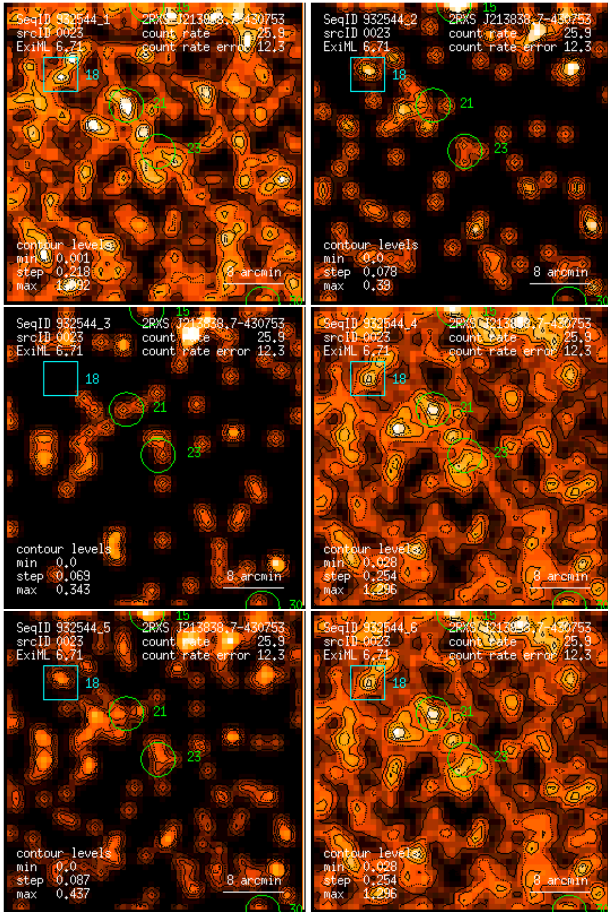
Figure 23: RASS 932544: detection 0023: band rate images, Gaussian filter: (1) PSPC channels 11 – 41, (2) 52 – 90, (3) 91 – 201, (4) 11 – 235, (5) 52 – 201, (6) 11 – 201. Broad band rates in counts/ks. Band rate contour levels in counts/ks/arcmin 2 .
