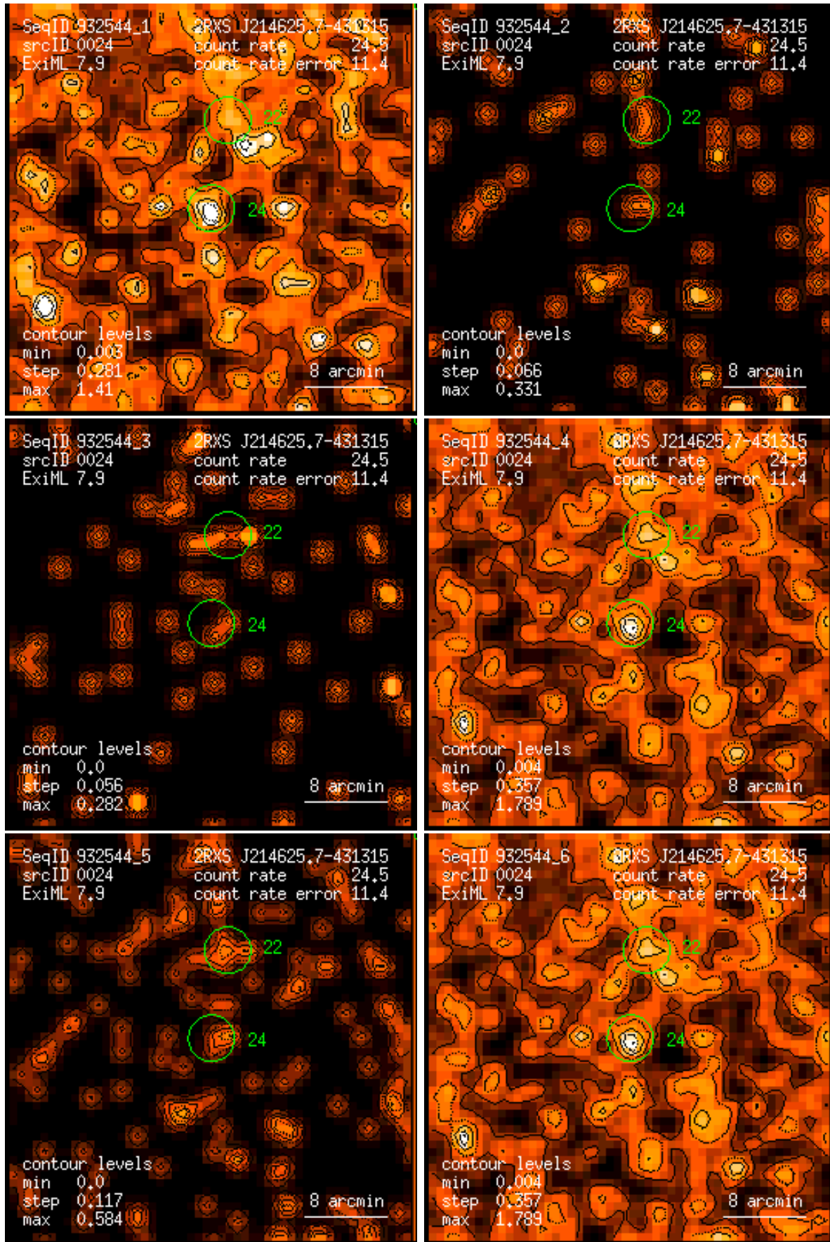
Figure 24: RASS 932544: detection 0024: band rate images, Gaussian filter: (1) PSPC channels 11 – 41, (2) 52 – 90, (3) 91 – 201, (4) 11 – 235, (5) 52 – 201, (6) 11 – 201. Broad band rates in counts/ks. Band rate contour levels in counts/ks/arcmin 2 .
