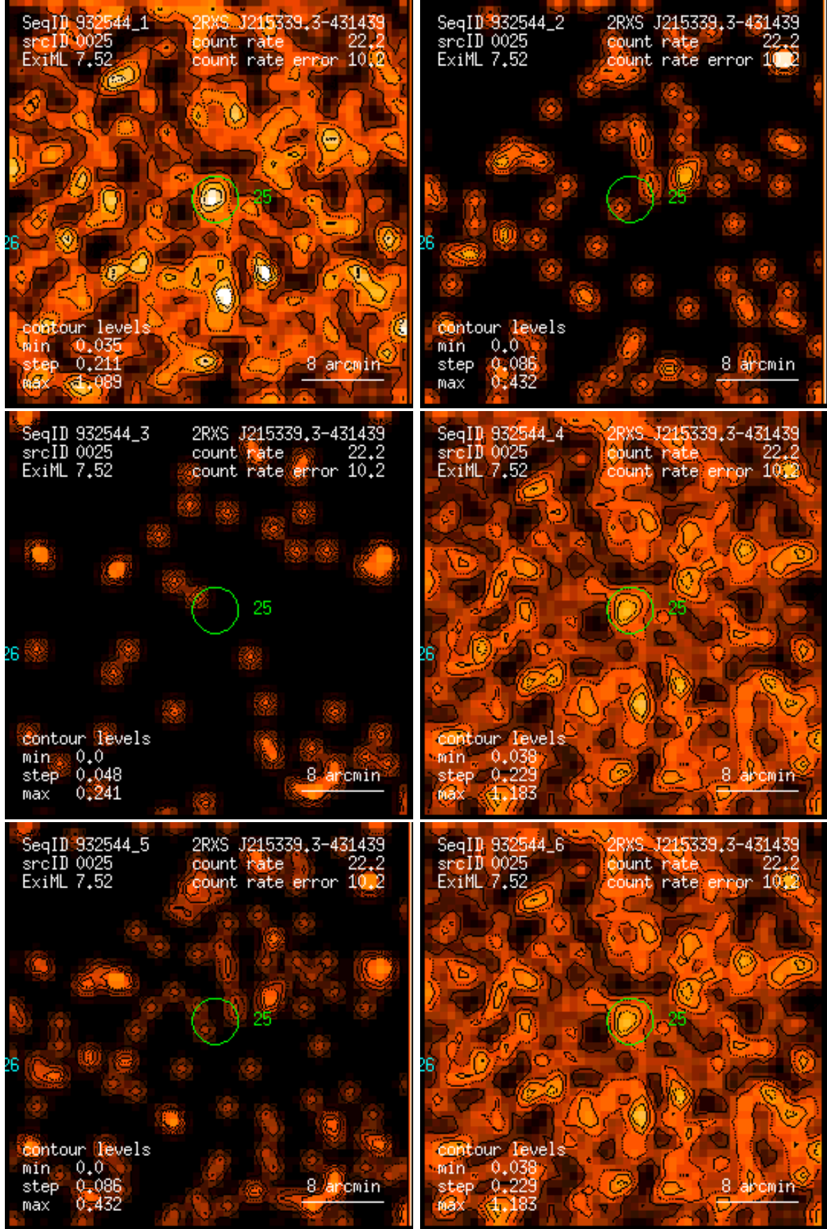
Figure 25: RASS 932544: detection 0025: band rate images, Gaussian filter: (1) PSPC channels 11 – 41, (2) 52 – 90, (3) 91 – 201, (4) 11 – 235, (5) 52 – 201, (6) 11 – 201. Broad band rates in counts/ks. Band rate contour levels in counts/ks/arcmin 2 .
