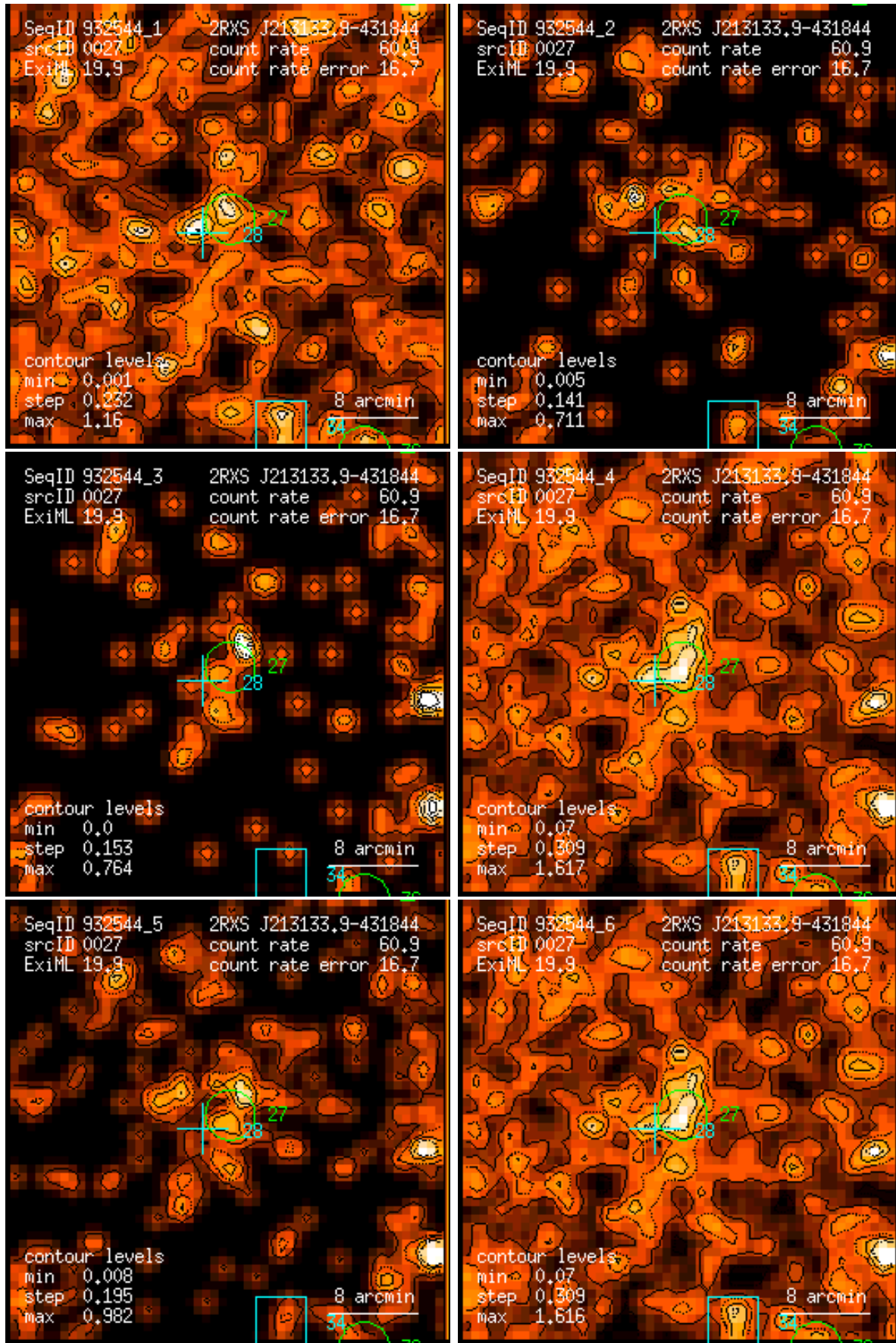
Figure 27: RASS 932544: detection 0027: band rate images, Gaussian filter: (1) PSPC channels 11 – 41, (2) 52 – 90, (3) 91 – 201, (4) 11 – 235, (5) 52 – 201, (6) 11 – 201. Broad band rates in counts/ks. Band rate contour levels in counts/ks/arcmin 2 .
