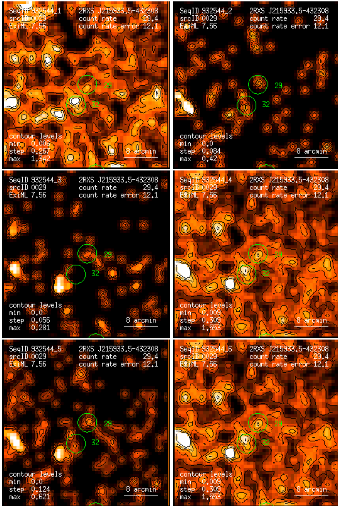
Figure 29: RASS 932544: detection 0029: band rate images, Gaussian filter: (1) PSPC channels 11 – 41, (2) 52 – 90, (3) 91 – 201, (4) 11 – 235, (5) 52 – 201, (6) 11 – 201. Broad band rates in counts/ks. Band rate contour levels in counts/ks/arcmin 2 .
