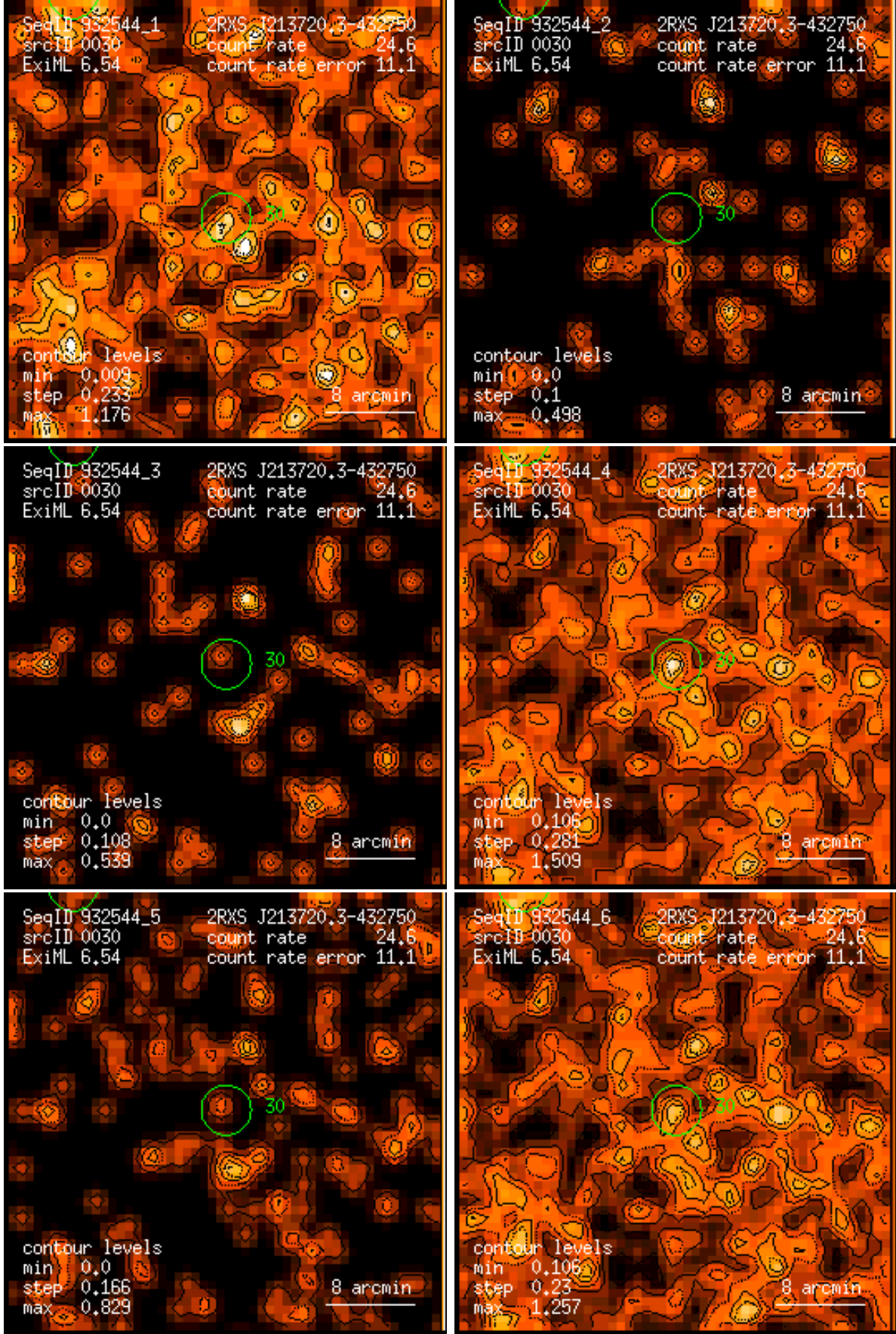
Figure 30: RASS 932544: detection 0030: band rate images, Gaussian filter: (1) PSPC channels 11 – 41, (2) 52 – 90, (3) 91 – 201, (4) 11 – 235, (5) 52 – 201, (6) 11 – 201. Broad band rates in counts/ks. Band rate contour levels in counts/ks/arcmin 2 .
