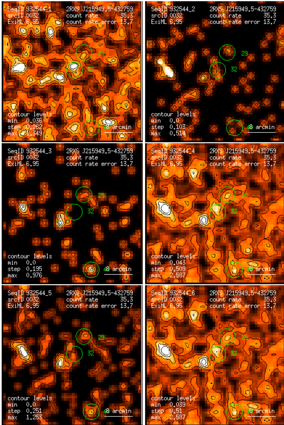
Figure 32: RASS 932544: detection 0032: band rate images, Gaussian filter: (1) PSPC channels 11 – 41, (2) 52 – 90, (3) 91 – 201, (4) 11 – 235, (5) 52 – 201, (6) 11 – 201. Broad band rates in counts/ks. Band rate contour levels in counts/ks/arcmin 2 .
