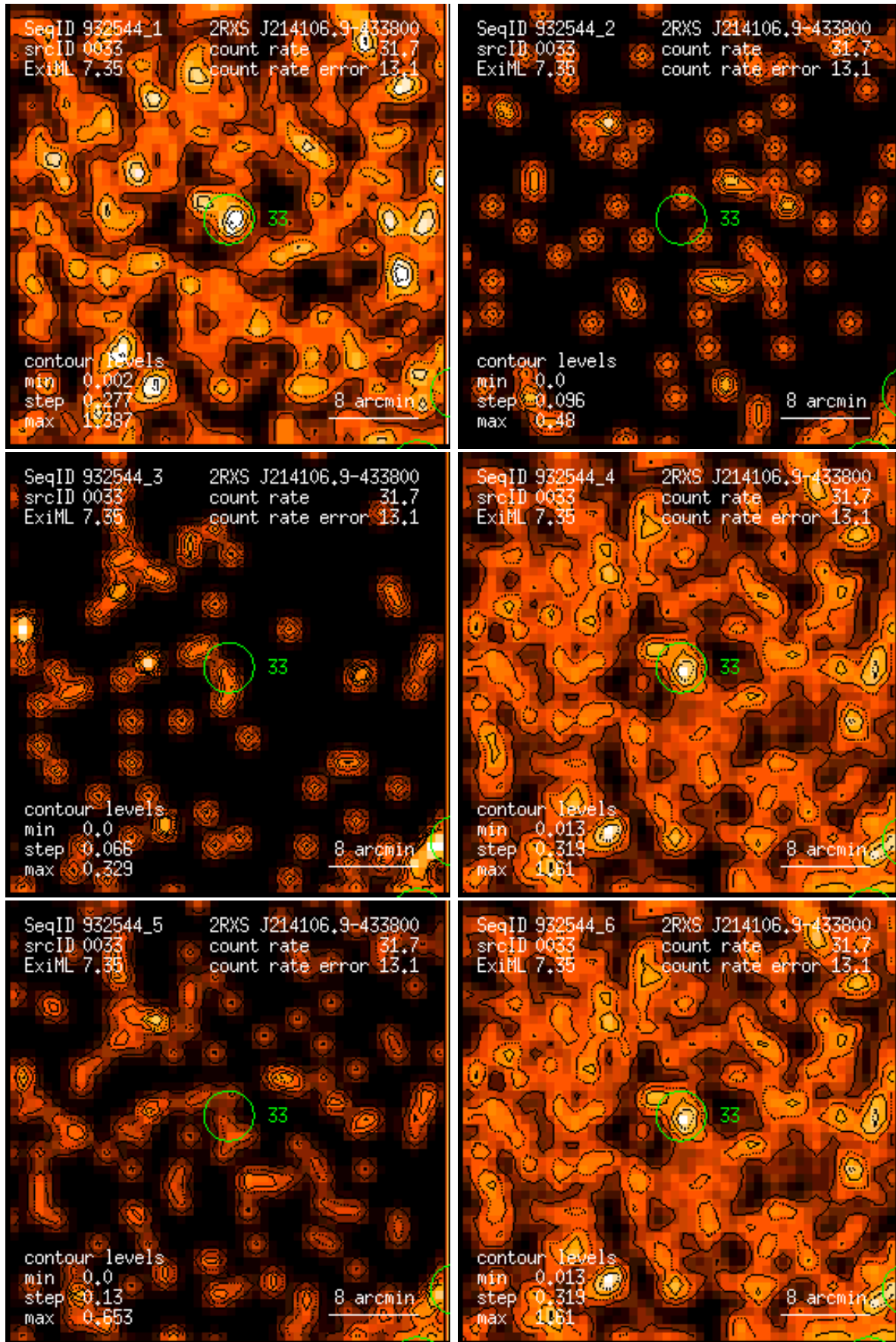
Figure 33: RASS 932544: detection 0033: band rate images, Gaussian filter: (1) PSPC channels 11 – 41, (2) 52 – 90, (3) 91 – 201, (4) 11 – 235, (5) 52 – 201, (6) 11 – 201. Broad band rates in counts/ks. Band rate contour levels in counts/ks/arcmin 2 .
