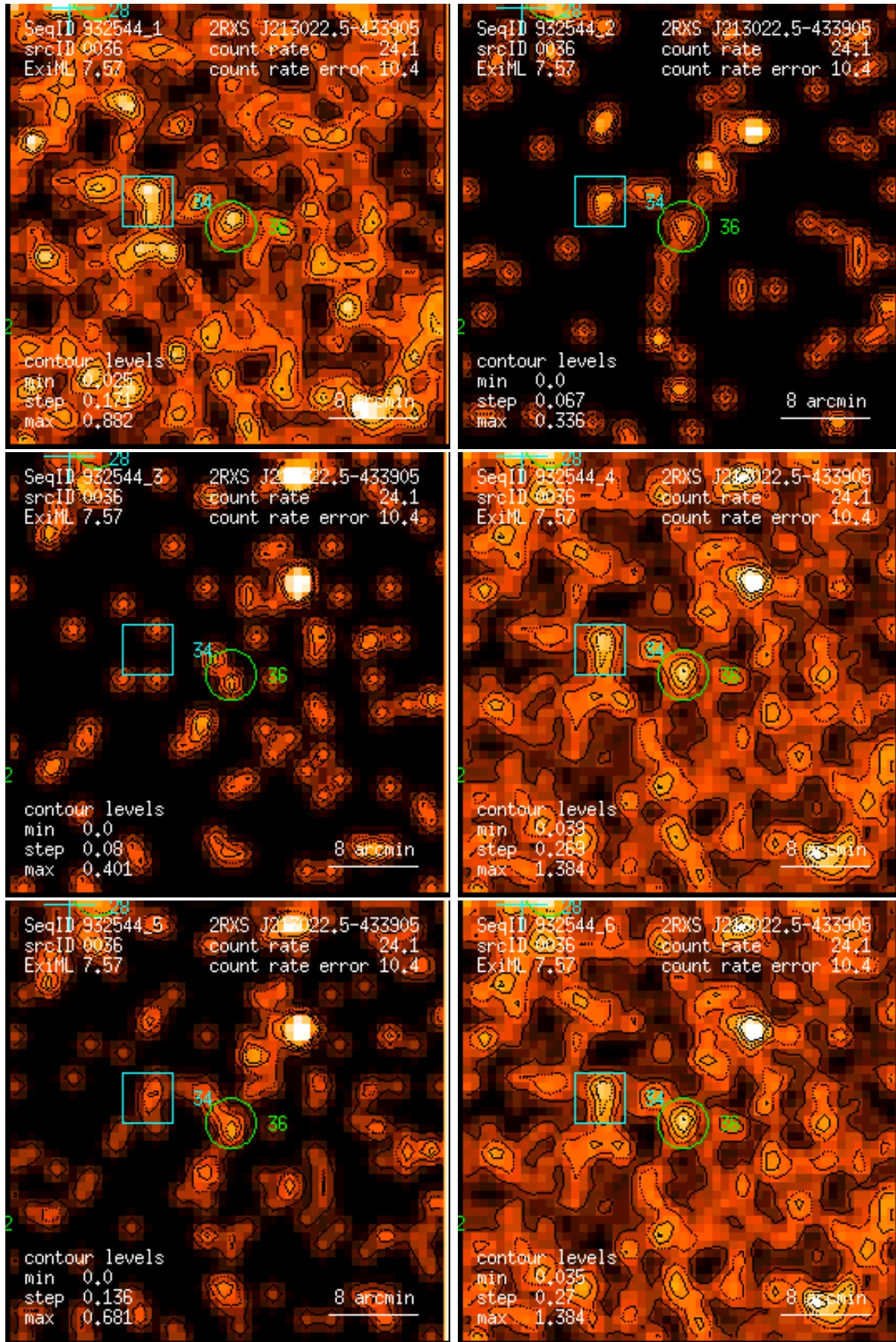
Figure 36: RASS 932544: detection 0036: band rate images, Gaussian filter: (1) PSPC channels 11 – 41, (2) 52 – 90, (3) 91 – 201, (4) 11 – 235, (5) 52 – 201, (6) 11 – 201. Broad band rates in counts/ks. Band rate contour levels in counts/ks/arcmin 2 .
