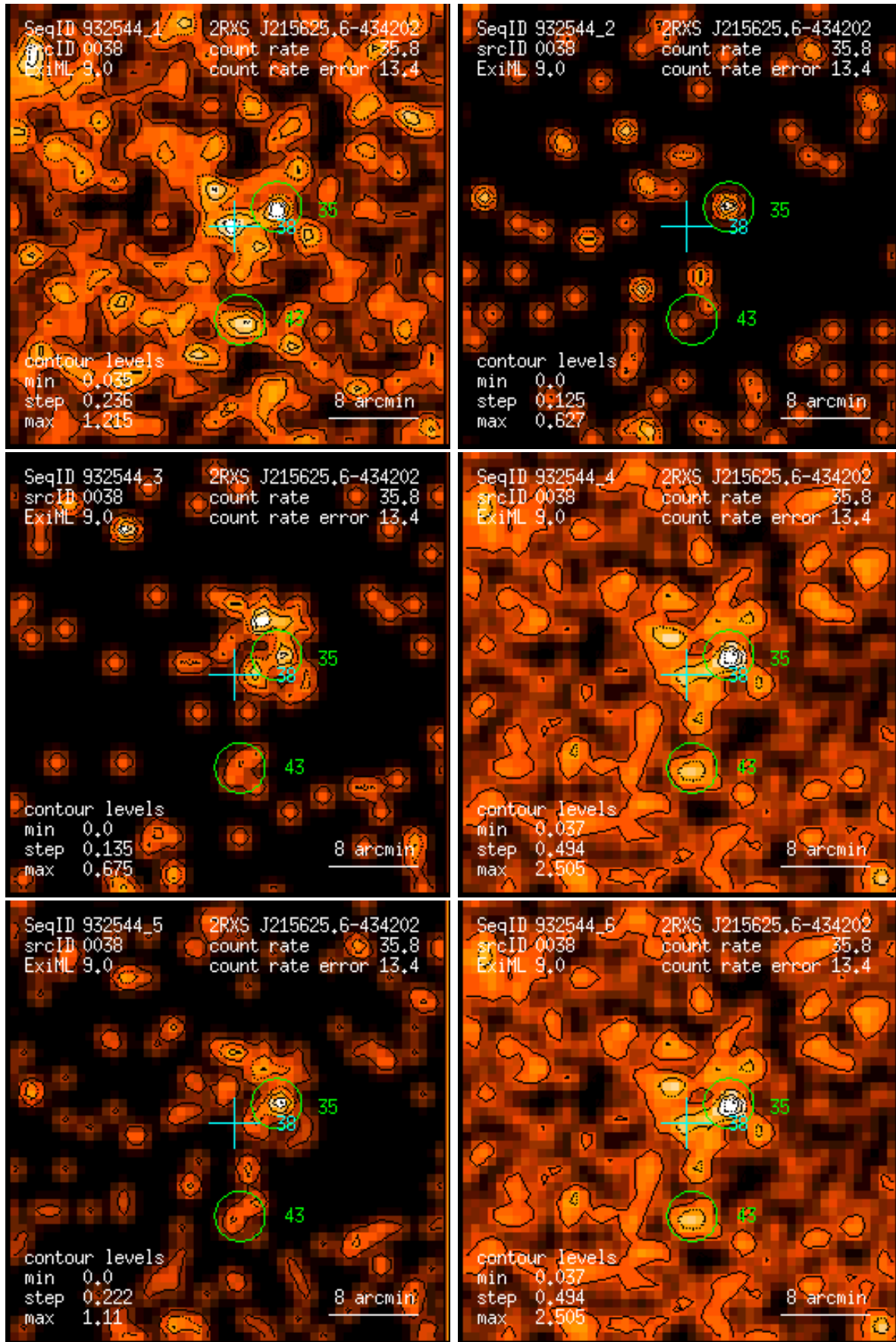
Figure 38: RASS 932544: detection 0038: band rate images, Gaussian filter: (1) PSPC channels 11 – 41, (2) 52 – 90, (3) 91 – 201, (4) 11 – 235, (5) 52 – 201, (6) 11 – 201. Broad band rates in counts/ks. Band rate contour levels in counts/ks/arcmin 2 .
