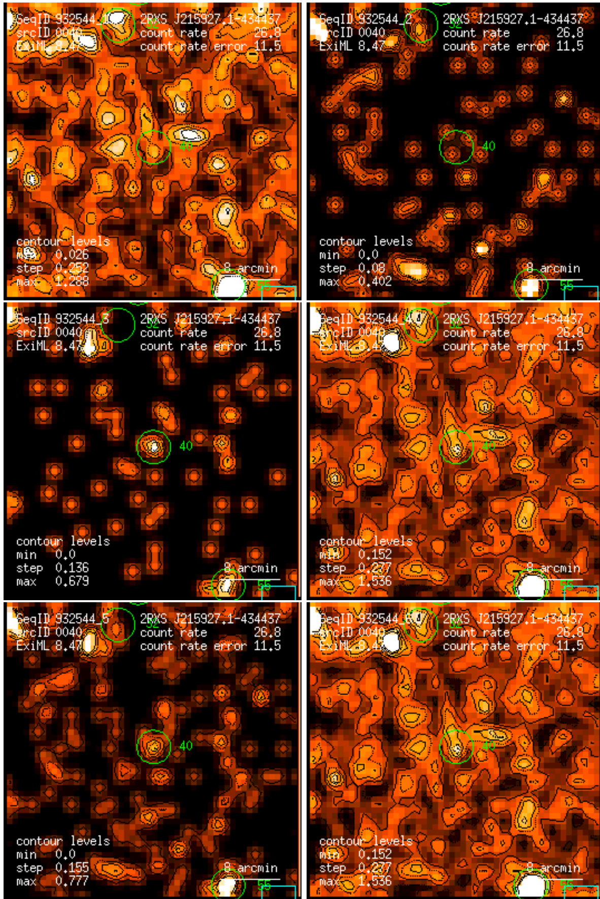
Figure 40: RASS 932544: detection 0040: band rate images, Gaussian filter: (1) PSPC channels 11 – 41, (2) 52 – 90, (3) 91 – 201, (4) 11 – 235, (5) 52 – 201, (6) 11 – 201. Broad band rates in counts/ks. Band rate contour levels in counts/ks/arcmin 2 .
