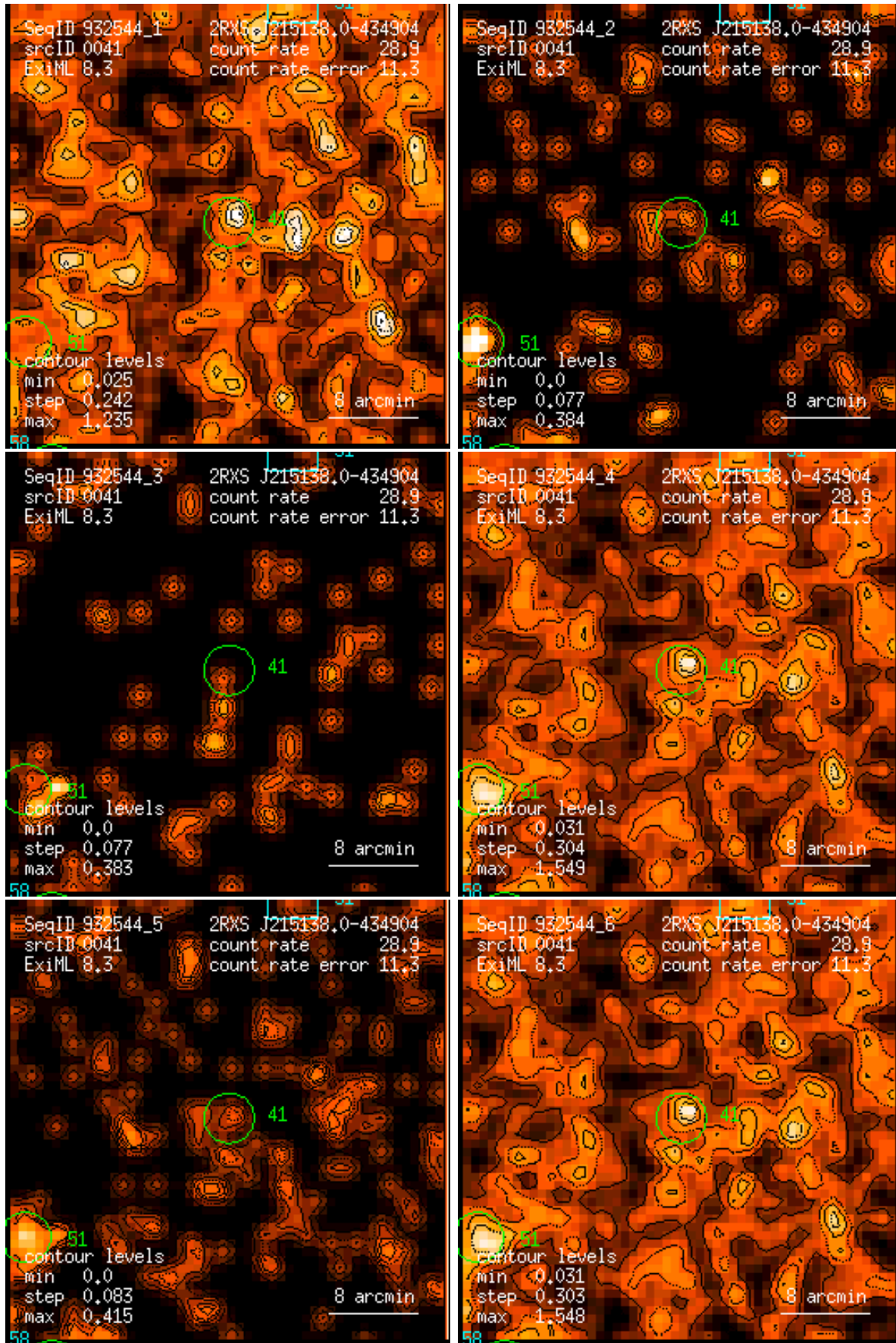
Figure 41: RASS 932544: detection 0041: band rate images, Gaussian filter: (1) PSPC channels 11 – 41, (2) 52 – 90, (3) 91 – 201, (4) 11 – 235, (5) 52 – 201, (6) 11 – 201. Broad band rates in counts/ks. Band rate contour levels in counts/ks/arcmin 2 .
