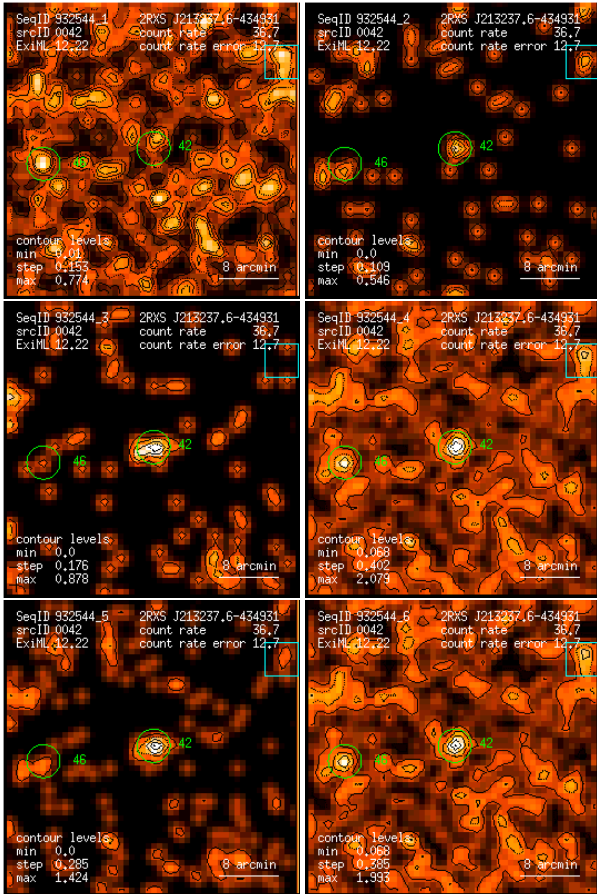
Figure 42: RASS 932544: detection 0042: band rate images, Gaussian filter: (1) PSPC channels 11 – 41, (2) 52 – 90, (3) 91 – 201, (4) 11 – 235, (5) 52 – 201, (6) 11 – 201. Broad band rates in counts/ks. Band rate contour levels in counts/ks/arcmin 2 .
