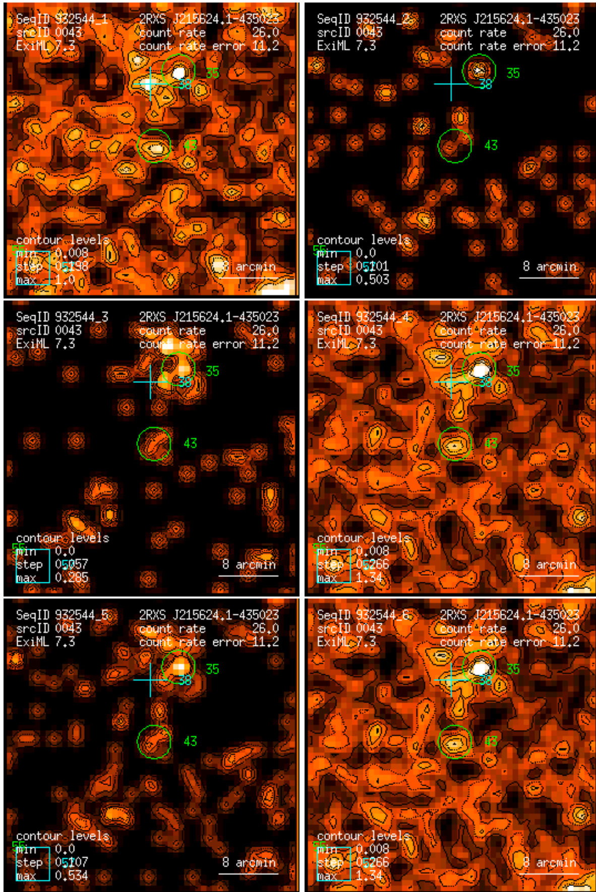
Figure 43: RASS 932544: detection 0043: band rate images, Gaussian filter: (1) PSPC channels 11 – 41, (2) 52 – 90, (3) 91 – 201, (4) 11 – 235, (5) 52 – 201, (6) 11 – 201. Broad band rates in counts/ks. Band rate contour levels in counts/ks/arcmin 2 .
