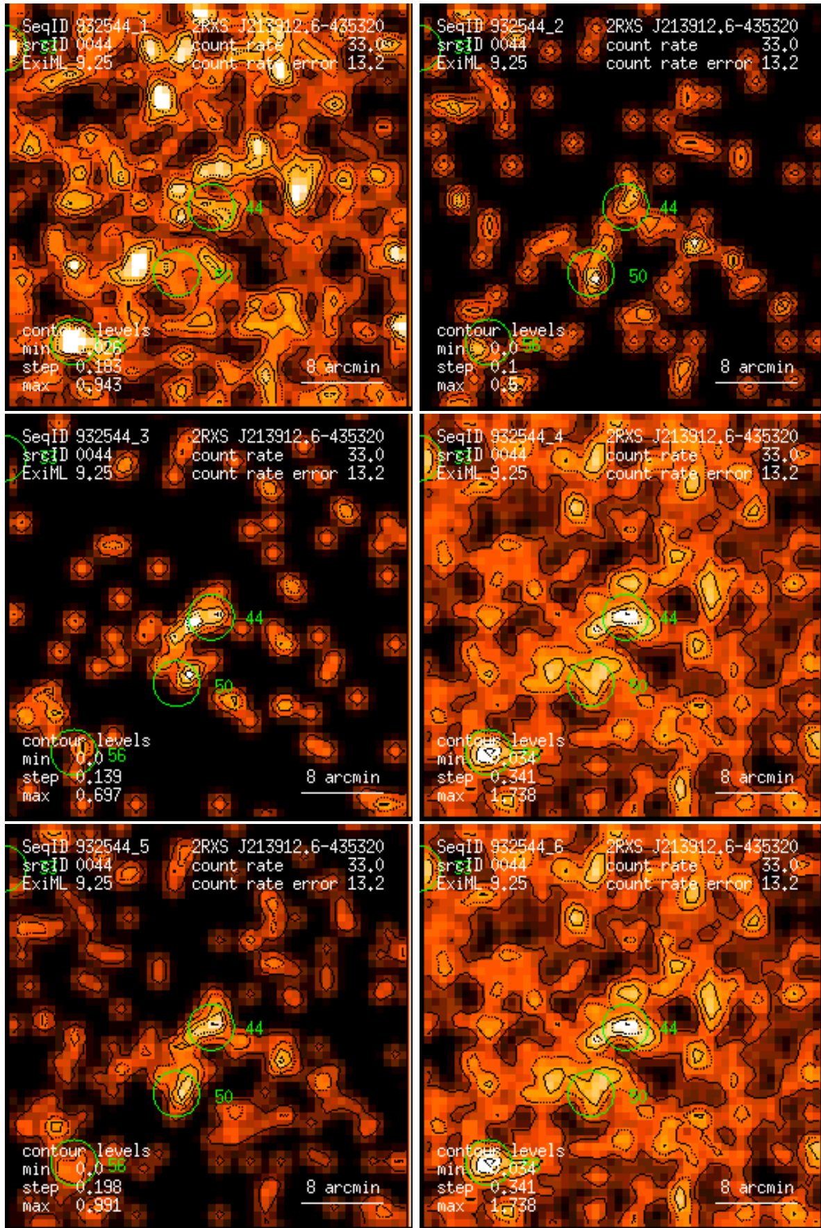
Figure 44: RASS 932544: detection 0044: band rate images, Gaussian filter: (1) PSPC channels 11 – 41, (2) 52 – 90, (3) 91 – 201, (4) 11 – 235, (5) 52 – 201, (6) 11 – 201. Broad band rates in counts/ks. Band rate contour levels in counts/ks/arcmin 2 .
